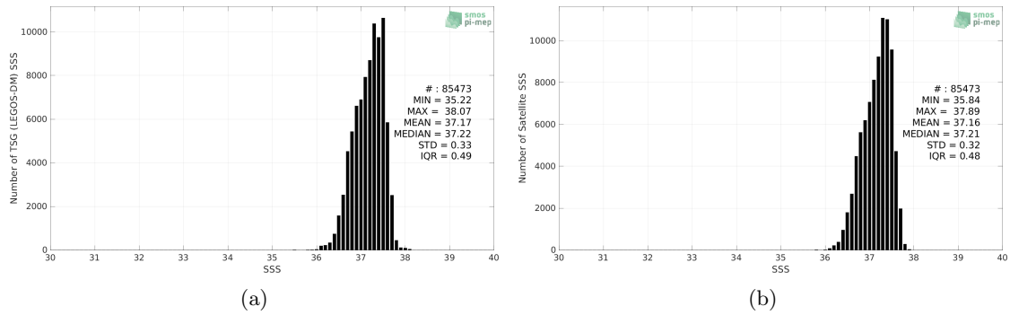
Figure 2: Histograms of SSS from TSG (LEGOS-DM) (a) and SMOS and SMAP SSS L4 OI v1 - 7 Days (LOPS) (b) considering all match-up pairs per bins of 0.1 over the SPURS 1 Pi-MEP region and for the full satellite product period.
