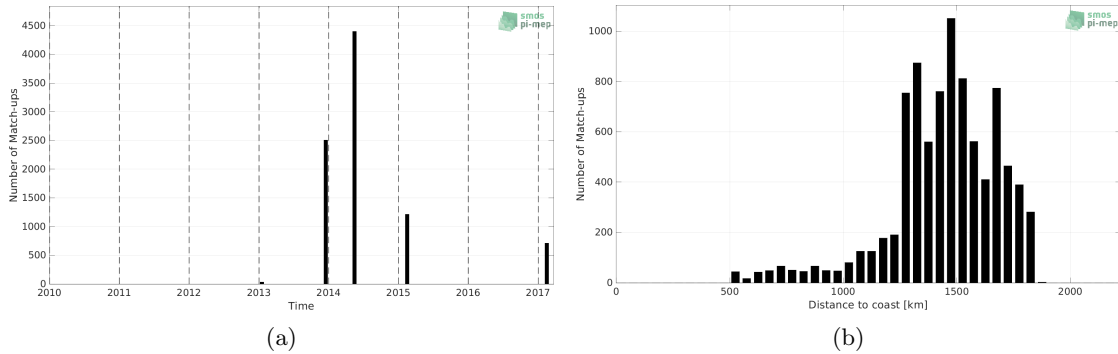
Figure 1: Number of match-ups between TSG (GOSUD-Sailing-ship) and SMOS and SMAP SSS L4 OI v1 - 7 Days (LOPS) SSS as a function of time (a) and as function of the distance to coast (b) over the SPURS 1 Pi-MEP region and for the full satellite product period.
