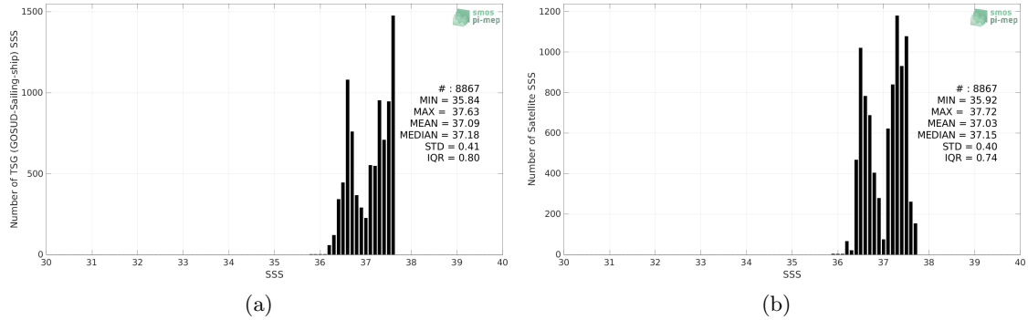
Figure 2: Histograms of SSS from TSG (GOSUD-Sailing-ship) (a) and SMOS and SMAP SSS L4 OI v1 - 7 Days (LOPS) (b) considering all match-up pairs per bins of 0.1 over the SPURS 1 Pi-MEP region and for the full satellite product period.
