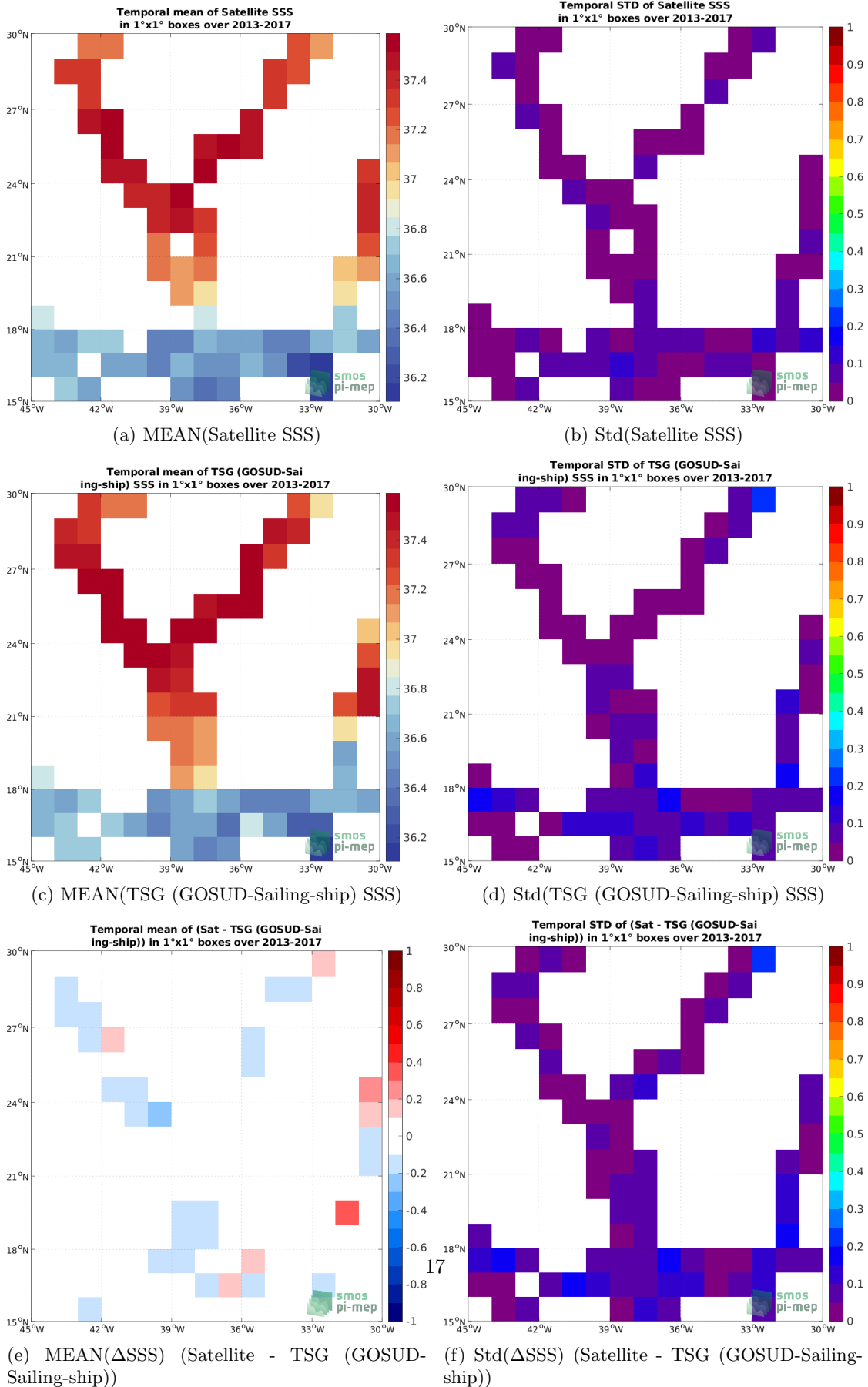
Figure 6: Temporal mean (left) and Std (right) of SSS from SMOS and SMAP SSS L4 OI v1 - 7 Days (LOPS) (top), TSG (GOSUD-Sailing-ship) (middle), and of \Delta SSS (Satellite - TSG (GOSUD-Sailing-ship)). Only match-up pairs are used to generate these maps.
