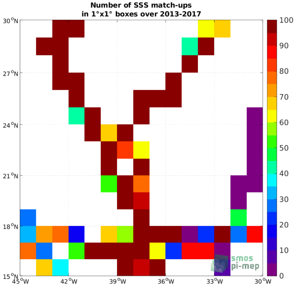
Figure 4: Number of SSS match-ups between TSG (GOSUD-Sailing-ship) SSS and the SMOS and SMAP SSS L4 OI v1 - 7 Days (LOPS) SSS product for the SPURS 1 Pi-MEP region over 1^\circ \times 1^\circ boxes and for the full satellite product period.
