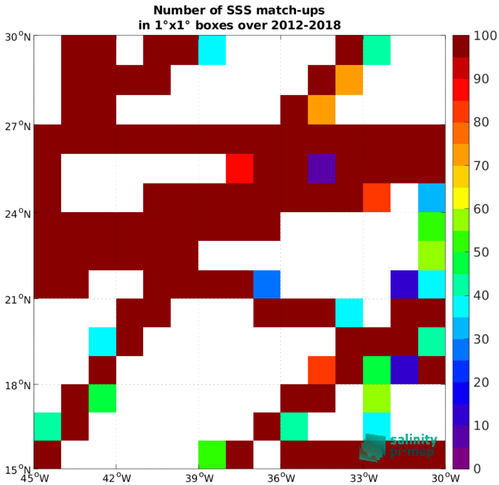
Figure 4: Number of SSS match-ups between TSG (GOSUD-Research-vessel) SSS and the SMOS and SMAP SSS L4 OI v1 - 7 Days (LOPS) SSS product for the SPURS 1 Pi-MEP region over 1°x1° boxes and for the full satellite product period.
