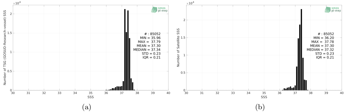
Figure 2: Histograms of SSS from TSG (GOSUD-Research-vessel) (a) and SMOS and SMAP SSS L4 OI v1 - 7 Days (LOPS) (b) considering all match-up pairs per bins of 0.1 over the SPURS 1 Pi-MEP region and for the full satellite product period.
