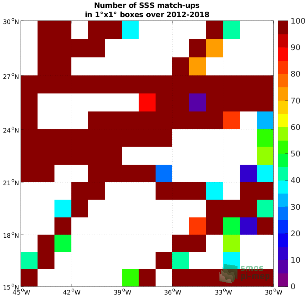
Figure 4: Number of SSS match-ups between TSG (GOSUD-Research-vessel) SSS and the SMOS and SMAP SSS L4 OI v1 - 7 Days (LOPS) SSS product for the SPURS 1 Pi-MEP region over 1^\circ \times 1^\circ boxes and for the full satellite product period.
