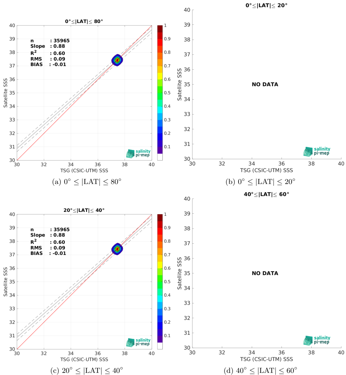
Figure 9: Contour maps of the concentration of SMOS and SMAP SSS L4 OI v1 - 7 Days (LOPS) SSS (y-axis) versus TSG (CSIC-UTM) SSS (x-axis) at match-up pairs for different latitude bands. For each plot, the red line shows x=y . The black thin and dashed lines indicate a linear fit through the data cloud and the \pm 95\% confidence levels, respectively. The number match-up pairs n , the slope and R^2 coefficient of the linear fit, the root mean square (RMS) and the mean bias between satellite and in situ data are indicated for each latitude band in each plots.
