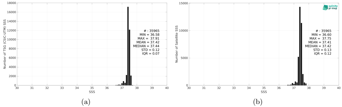
Figure 2: Histograms of SSS from TSG (CSIC-UTM) (a) and SMOS and SMAP SSS L4 OI v1 - 7 Days (LOPS) (b) considering all match-up pairs per bins of 0.1 over the SPURS 1 Pi-MEP region and for the full satellite product period.
