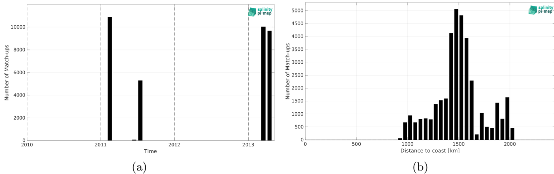
Figure 1: Number of match-ups between TSG (CSIC-UTM) and SMOS and SMAP SSS L4 OI v1 - 7 Days (LOPS) SSS as a function of time (a) and as function of the distance to coast (b) over the SPURS 1 Pi-MEP region and for the full satellite product period.
