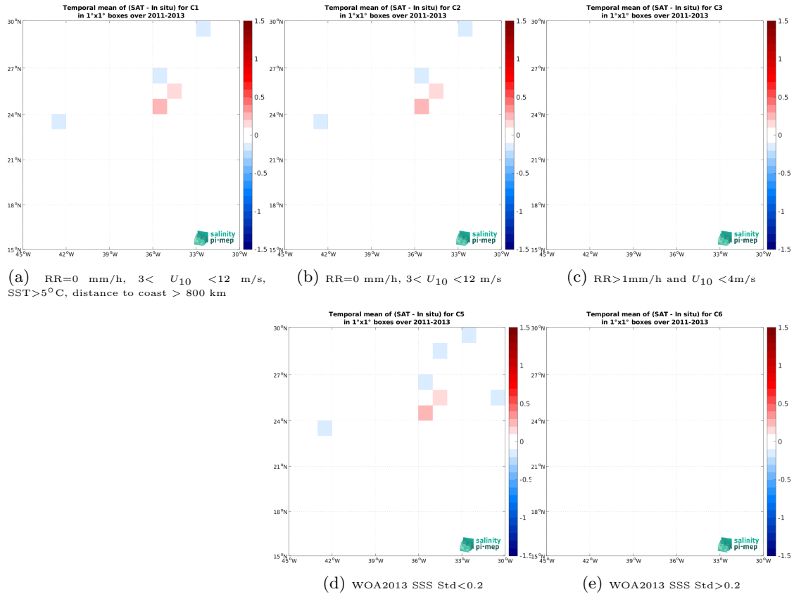
Figure 12: Temporal mean gridded over spatial boxes of size 1^{\circ}\times 1^{\circ} of \Delta\text{SSS} (SMOS and SMAP SSS L4 OI v1 - 7 Days (LOPS) - TSG (CSIC-UTM)) for 5 different subdatasets corresponding to:RR=0 mm/h, 3 < U_{10} < 12 m/s, SST >5^{\circ}\text{C} , distance to coast > 800 km (a), RR=0 mm/h, 3 < U_{10} < 12 m/s (b), RR >1 mm/h and U_{10} < 4 m/s (c), WOA2013 SSS Std <0.2 (d), WOA2013 SSS Std >0.2 (e).
