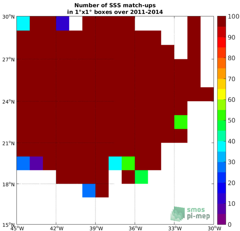
Figure 3: Number of SSS match-ups between Surface drifters SSS and the SMOS and SMAP SSS L4 OI v1 - 7 Days (LOPS) SSS product for the SPURS 1 Pi-MEP region over 1°x1° boxes and for the full satellite product period.
