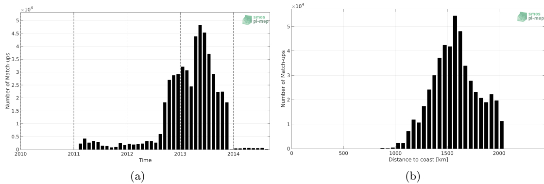
Figure 1: Number of match-ups between Surface drifters and SMOS and SMAP SSS L4 OI v1 - 7 Days (LOPS) SSS as a function of time (a) and as function of the distance to coast (b) over the SPURS 1 Pi-MEP region and for the full satellite product period.
