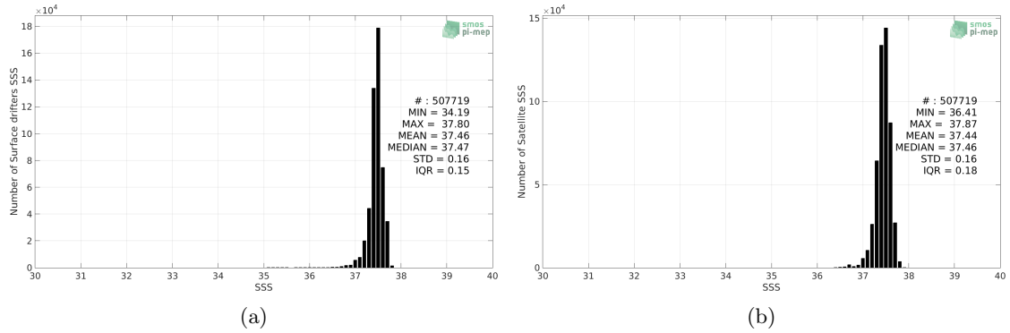
Figure 2: Histograms of SSS from Surface drifters (a) and SMOS and SMAP SSS L4 OI v1 - 7 Days (LOPS) (b) considering all match-up pairs per bins of 0.1 over the SPURS 1 Pi-MEP region and for the full satellite product period.
