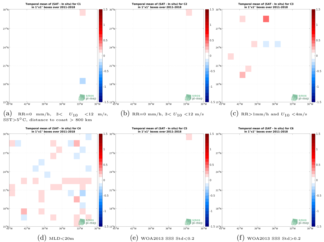
Figure 12: Temporal mean gridded over spatial boxes of size 1^\circ \times 1^\circ of \Delta SSS (SMOS and SMAP SSS L4 OI v1 - 7 Days (LOPS) - Argo) for 6 different subdatasets corresponding to:RR=0 mm/h, 3 < U_{10} < 12 m/s, SST >5^\circ C, distance to coast > 800 km (a), RR=0 mm/h, 3 < U_{10} < 12 m/s (b), RR >1 mm/h and U_{10} < 4 m/s (c),MLD <20 m (d),WOA2013 SSS Std <0.2 (e),WOA2013 SSS Std >0.2 (f).
