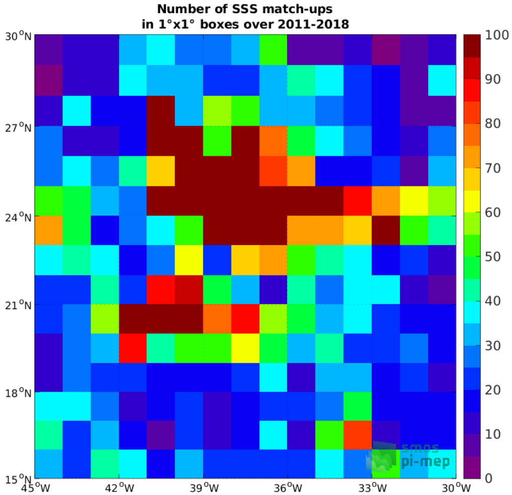
Figure 4: Number of SSS match-ups between Argo SSS and the SMOS and SMAP SSS L4 OI v1 - 7 Days (LOPS) SSS product for the SPURS 1 Pi-MEP region over 1^\circ \times 1^\circ boxes and for the full satellite product period.
