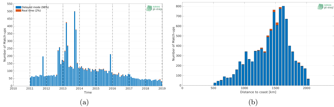
Figure 1: Number of match-ups between Argo and SMOS and SMAP SSS L4 OI v1 - 7 Days (LOPS) SSS as a function of time (a) and as function of the distance to coast (b) over the SPURS 1 Pi-MEP region and for the full satellite product period.
