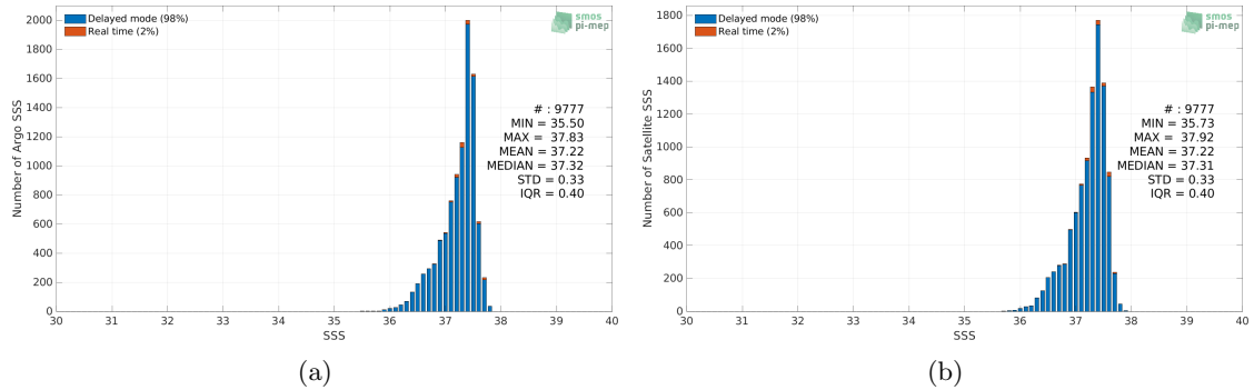
Figure 2: Histograms of SSS from Argo (a) and SMOS and SMAP SSS L4 OI v1 - 7 Days (LOPS) (b) considering all match-up pairs per bins of 0.1 over the SPURS 1 Pi-MEP region and for the full satellite product period.
