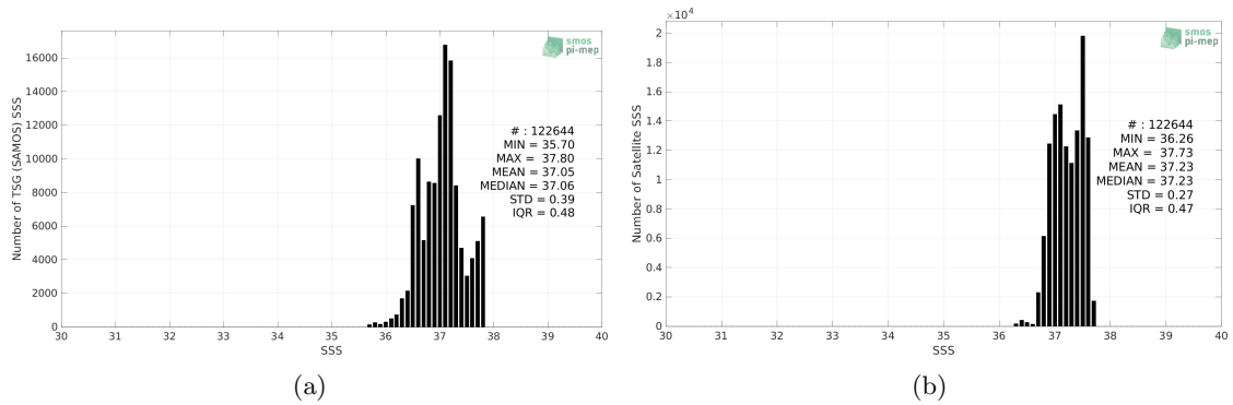
Figure 2: Histograms of SSS from TSG (SAMOS) (a) and SMOS SSS L4 v1 - Weekly (CMEMS-CNR) (b) considering all match-up pairs per bins of 0.1 over the SPURS 1 Pi-MEP region and for the full satellite product period.
