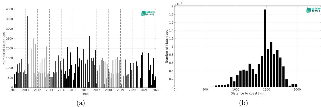
Figure 1: Number of match-ups between TSG (LEGOS-DM) and SMOS SSS L4 v1 - Weekly (CMEMS-CNR) SSS as a function of time (a) and as function of the distance to coast (b) over the SPURS 1 Pi-MEP region and for the full satellite product period.
