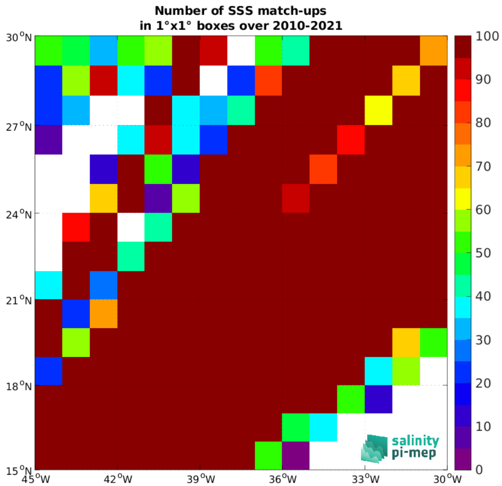
Figure 4: Number of SSS match-ups between TSG (LEGOS-DM) SSS and the SMOS SSS L4 v1 - Weekly (CMEMS-CNR) SSS product for the SPURS 1 Pi-MEP region over 1^\circ \times 1^\circ boxes and for the full satellite product period.
