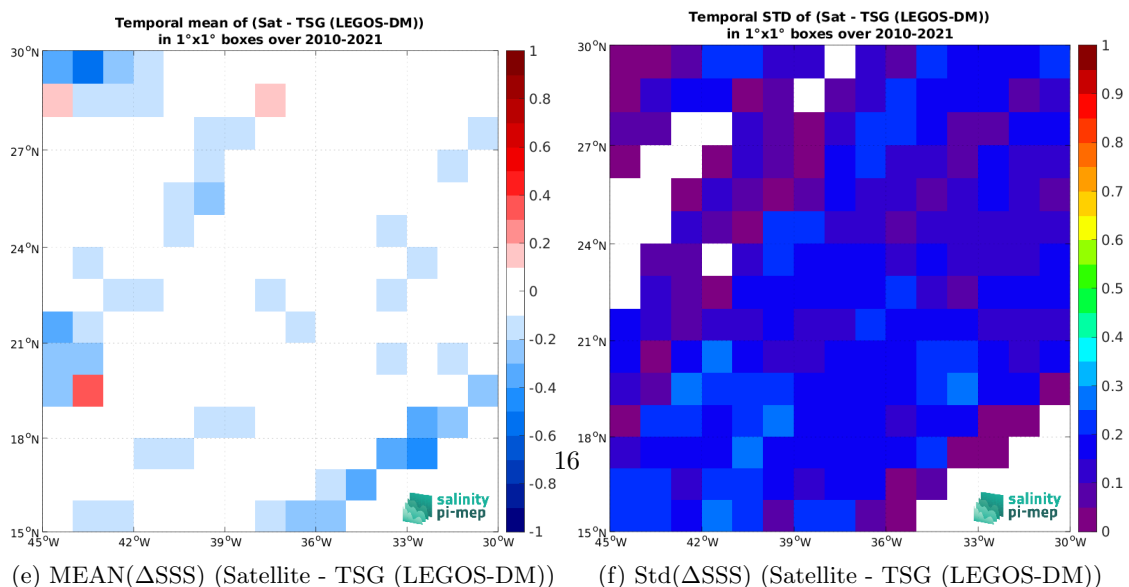
Figure 6: Temporal mean (left) and Std (right) of SSS from SMOS SSS L4 v1 - Weekly (CMEMS-CNR) (top), TSG (LEGOS-DM) (middle), and of \Delta SSS (Satellite - TSG (LEGOS-DM)). Only match-up pairs are used to generate these maps.
