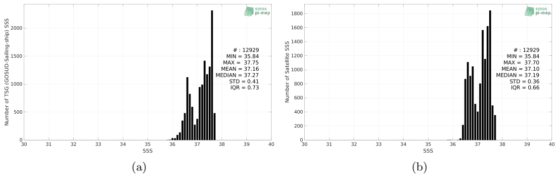
Figure 2: Histograms of SSS from TSG (GOSUD-Sailing-ship) (a) and SMOS SSS L4 v1 - Weekly (CMEMS-CNR) (b) considering all match-up pairs per bins of 0.1 over the SPURS 1 Pi-MEP region and for the full satellite product period.
