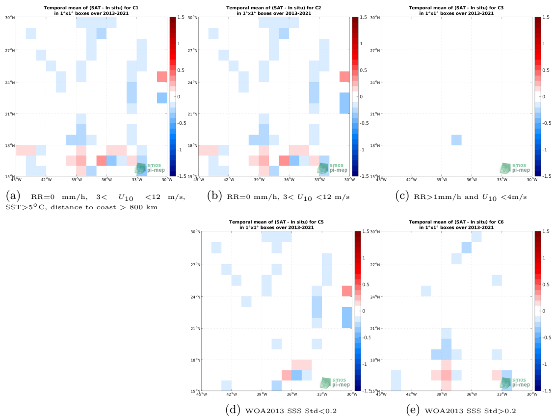
Figure 12: Temporal mean gridded over spatial boxes of size 1^\circ \times 1^\circ of \Delta SSS (SMOS SSS L4 v1 - Weekly (CMEMS-CNR) - TSG (GOSUD-Sailing-ship)) for 5 different subdatasets corresponding to: RR=0 mm/h, 3 < U_{10} < 12 m/s, SST > 5^\circ C , distance to coast > 800 km (a), RR=0 mm/h, 3 < U_{10} < 12 m/s (b), RR > 1 mm/h and U_{10} < 4 m/s (c), WOA2013 SSS Std < 0.2 (d), WOA2013 SSS Std > 0.2 (e).
