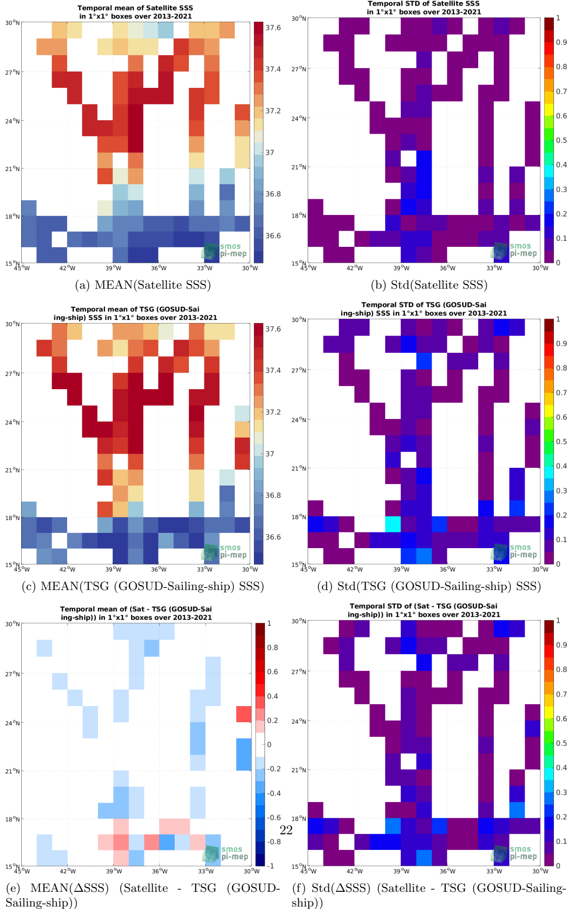
Figure 6: Temporal mean (left) and Std (right) of SSS from SMOS SSS L4 v1 - Weekly (CMEMS-CNR) (top), TSG (GOSUD-Sailing-ship) (middle), and of \Delta SSS (Satellite - TSG (GOSUD-Sailing-ship)). Only match-up pairs are used to generate these maps.
