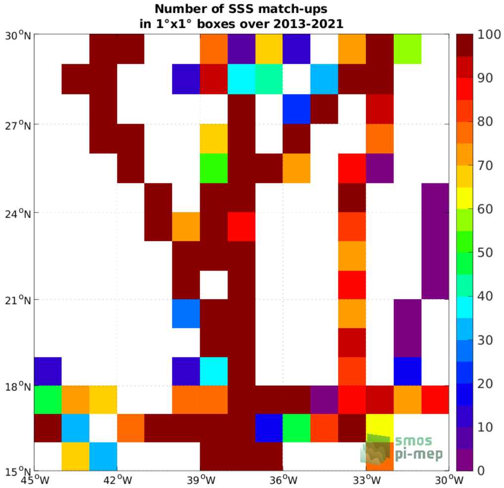
Figure 4: Number of SSS match-ups between TSG (GOSUD-Sailing-ship) SSS and the SMOS SSS L4 v1 - Weekly (CMEMS-CNR) SSS product for the SPURS 1 Pi-MEP region over 1°x1° boxes and for the full satellite product period.
