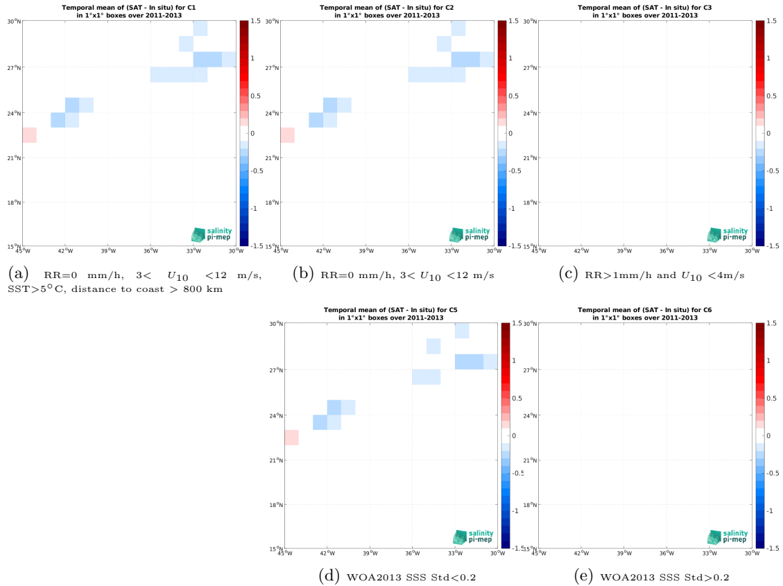
Figure 12: Temporal mean gridded over spatial boxes of size 1^{\circ}\times 1^{\circ} of \Delta\text{SSS} (SMOS SSS L4 v1 - Weekly (CMEMS-CNR) - TSG (CSIC-UTM)) for 5 different subdatasets corresponding to:RR=0 mm/h, 3 < U_{10} < 12 m/s, SST >5^{\circ}\text{C} , distance to coast > 800 km (a), RR=0 mm/h, 3 < U_{10} < 12 m/s (b), RR >1 mm/h and U_{10} < 4 m/s (c), WOA2013 SSS Std <0.2 (d), WOA2013 SSS Std >0.2 (e).
