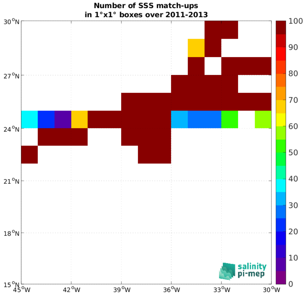
Figure 4: Number of SSS match-ups between TSG (CSIC-UTM) SSS and the SMOS SSS L4 v1 - Weekly (CMEMS-CNR) SSS product for the SPURS 1 Pi-MEP region over 1^\circ \times 1^\circ boxes and for the full satellite product period.
