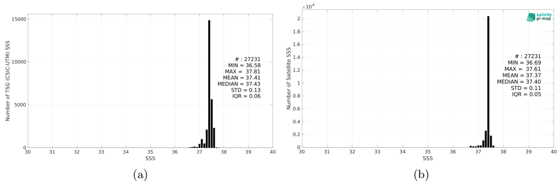
Figure 2: Histograms of SSS from TSG (CSIC-UTM) (a) and SMOS SSS L4 v1 - Weekly (CMEMS-CNR) (b) considering all match-up pairs per bins of 0.1 over the SPURS 1 Pi-MEP region and for the full satellite product period.
