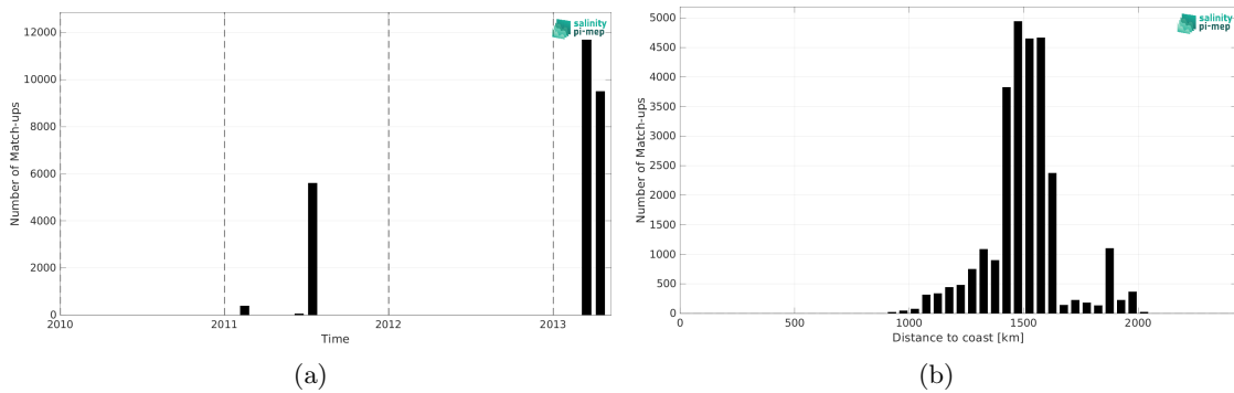
Figure 1: Number of match-ups between TSG (CSIC-UTM) and SMOS SSS L4 v1 - Weekly (CMEMS-CNR) SSS as a function of time (a) and as function of the distance to coast (b) over the SPURS 1 Pi-MEP region and for the full satellite product period.
