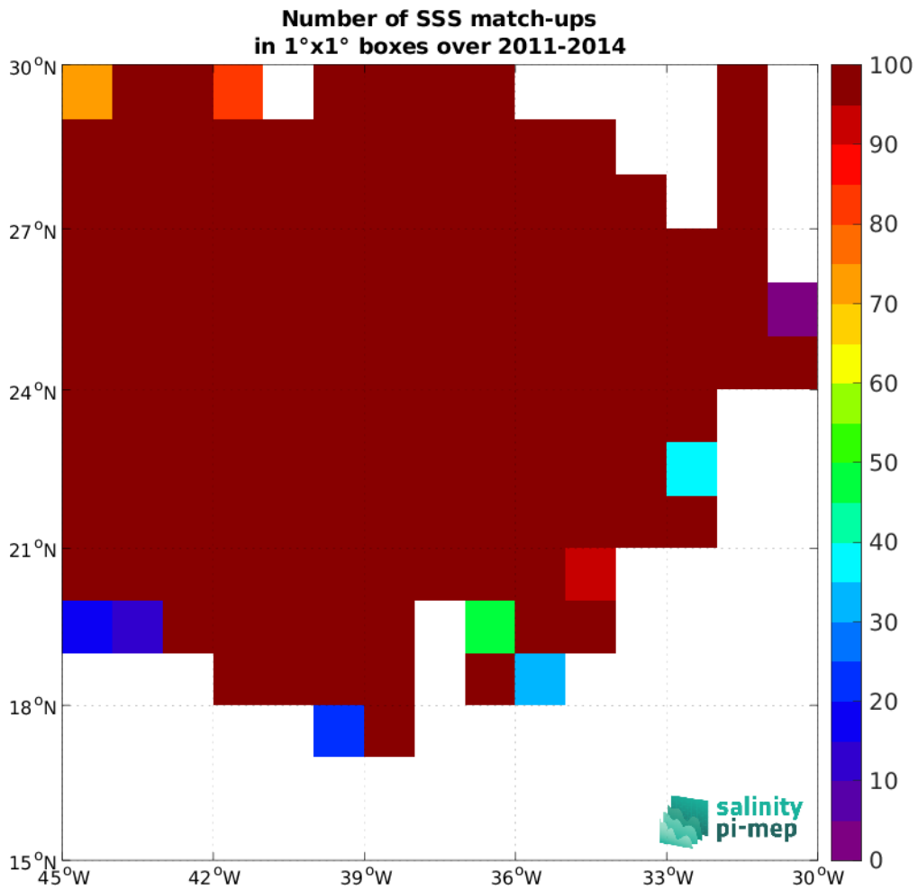
Figure 3: Number of SSS match-ups between Surface drifters SSS and the SMOS SSS L4 v1 - Weekly (CMEMS-CNR) SSS product for the SPURS 1 Pi-MEP region over 1°×1° boxes and for the full satellite product period.
