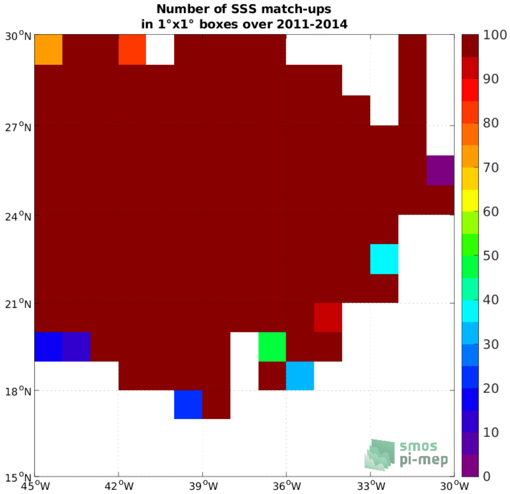
Figure 3: Number of SSS match-ups between Surface drifters SSS and the SMOS SSS L4 v1 - Weekly (CMEMS-CNR) SSS product for the SPURS 1 Pi-MEP region over 1^\circ \times 1^\circ boxes and for the full satellite product period.
