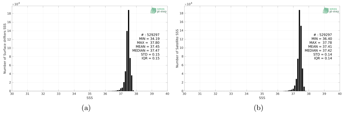
Figure 2: Histograms of SSS from Surface drifters (a) and SMOS SSS L4 v1 - Weekly (CMEMS-CNR) (b) considering all match-up pairs per bins of 0.1 over the SPURS 1 Pi-MEP region and for the full satellite product period.
