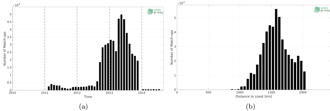
Figure 1: Number of match-ups between Surface drifters and SMOS SSS L4 v1 - Weekly (CMEMS-CNR) SSS as a function of time (a) and as function of the distance to coast (b) over the SPURS 1 Pi-MEP region and for the full satellite product period.
