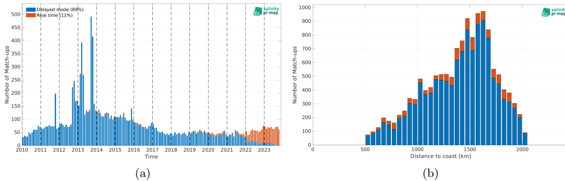
Figure 1: Number of match-ups between Argo and SMOS SSS L4 v1 - Weekly (CMEMS-CNR) SSS as a function of time (a) and as function of the distance to coast (b) over the SPURS 1 Pi-MEP region and for the full satellite product period.
