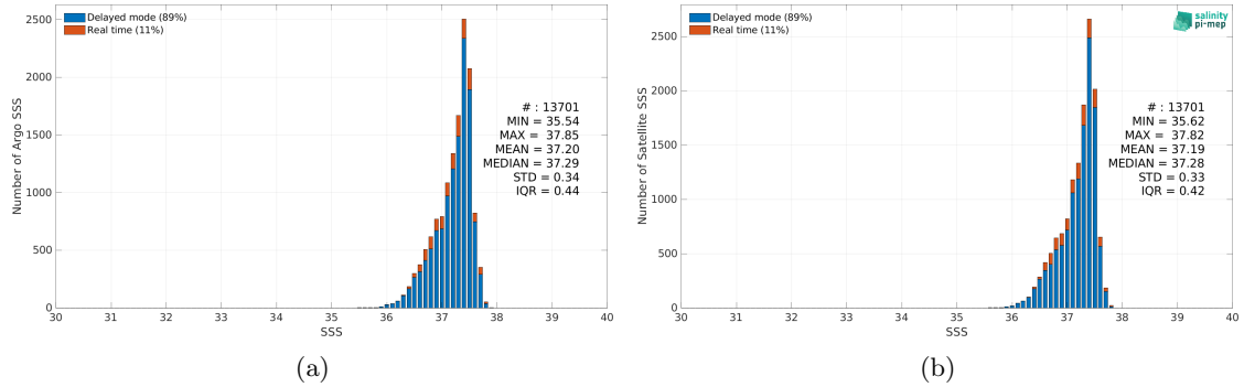
Figure 2: Histograms of SSS from Argo (a) and SMOS SSS L4 v1 - Weekly (CMEMS-CNR) (b) considering all match-up pairs per bins of 0.1 over the SPURS 1 Pi-MEP region and for the full satellite product period.
