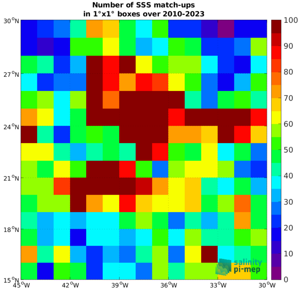
Figure 4: Number of SSS match-ups between Argo SSS and the SMOS SSS L4 v1 - Weekly (CMEMS-CNR) SSS product for the SPURS 1 Pi-MEP region over 1^\circ \times 1^\circ boxes and for the full satellite product period.
