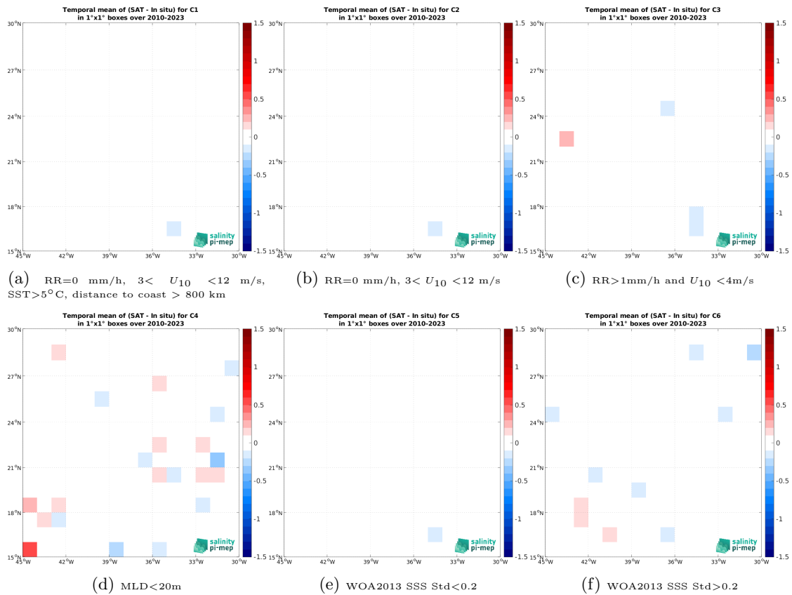
Figure 12: Temporal mean gridded over spatial boxes of size 1^\circ \times 1^\circ of \Delta SSS (SMOS SSS L4 v1 - Weekly (CMEMS-CNR) - Argo) for 6 different subdatasets corresponding to:RR=0 mm/h, 3 < U_{10} < 12 m/s, SST >5^\circ\text{C} , distance to coast > 800 km (a), RR=0 mm/h, 3 < U_{10} < 12 m/s (b), RR >1 mm/h and U_{10} < 4 m/s (c),MLD <20 m (d),WOA2013 SSS Std <0.2 (e),WOA2013 SSS Std >0.2 (f).
