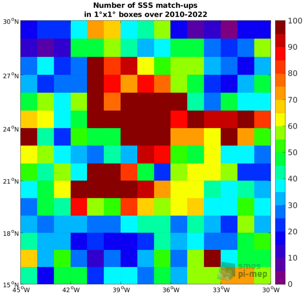
Figure 4: Number of SSS match-ups between Argo SSS and the SMOS SSS L4 v1 - Weekly (CMEMS-CNR) SSS product for the SPURS 1 Pi-MEP region over 1°×1° boxes and for the full satellite product period.
