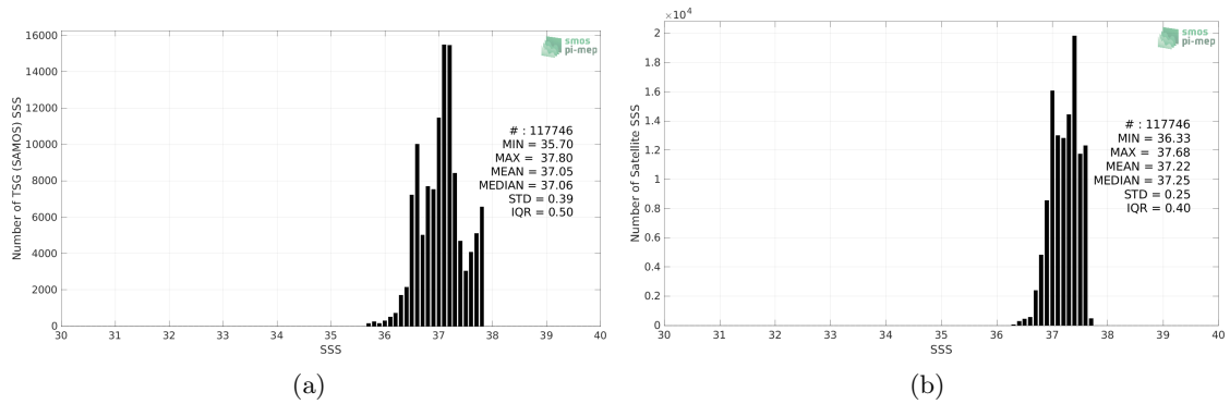
Figure 2: Histograms of SSS from TSG (SAMOS) (a) and SMOS SSS L4 v1 - Monthly (CMEMS-CNR) (b) considering all match-up pairs per bins of 0.1 over the SPURS 1 Pi-MEP region and for the full satellite product period.
