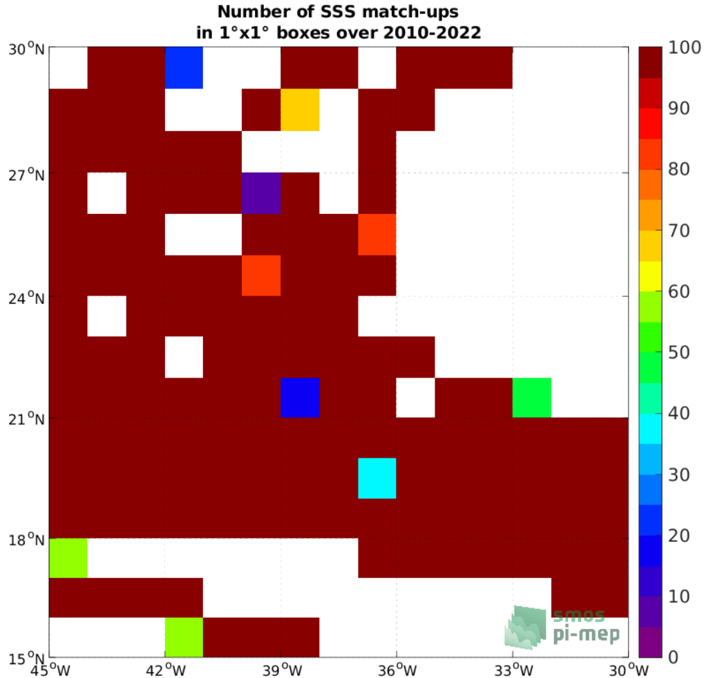
Figure 4: Number of SSS match-ups between TSG (SAMOS) SSS and the SMOS SSS L4 v1 - Monthly (CMEMS-CNR) SSS product for the SPURS 1 Pi-MEP region over 1^\circ \times 1^\circ boxes and for the full satellite product period.
