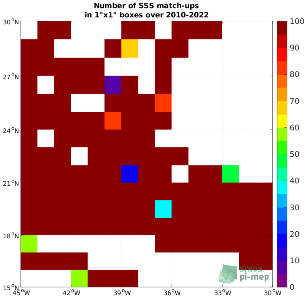
Figure 4: Number of SSS match-ups between TSG (SAMOS) SSS and the SMOS SSS L4 v1 - Monthly (CMEMS-CNR) SSS product for the SPURS 1 Pi-MEP region over 1°x1° boxes and for the full satellite product period.
