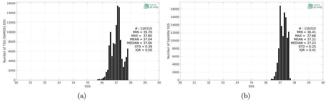
Figure 2: Histograms of SSS from TSG (SAMOS) (a) and SMOS SSS L4 v1 - Monthly (CMEMS-CNR) (b) considering all match-up pairs per bins of 0.1 over the SPURS 1 Pi-MEP region and for the full satellite product period.
