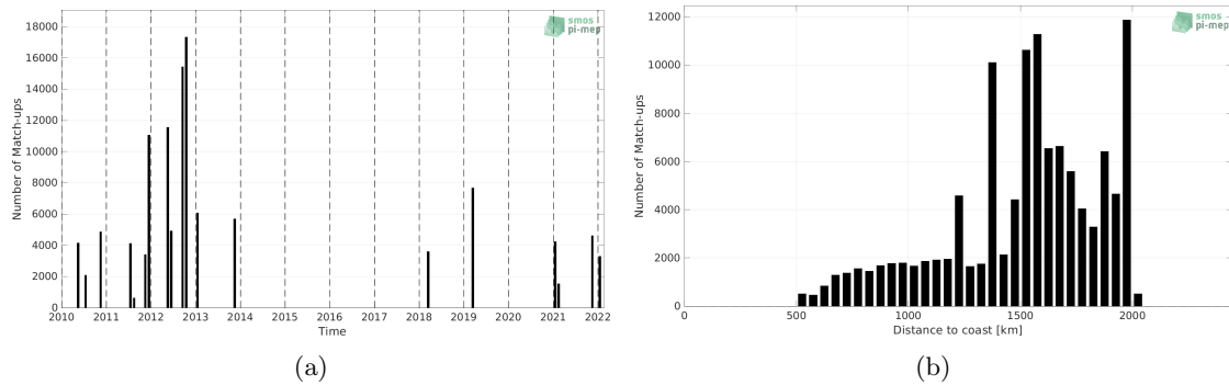
Figure 1: Number of match-ups between TSG (SAMOS) and SMOS SSS L4 v1 - Monthly (CMEMS-CNR) SSS as a function of time (a) and as function of the distance to coast (b) over the SPURS 1 Pi-MEP region and for the full satellite product period.
