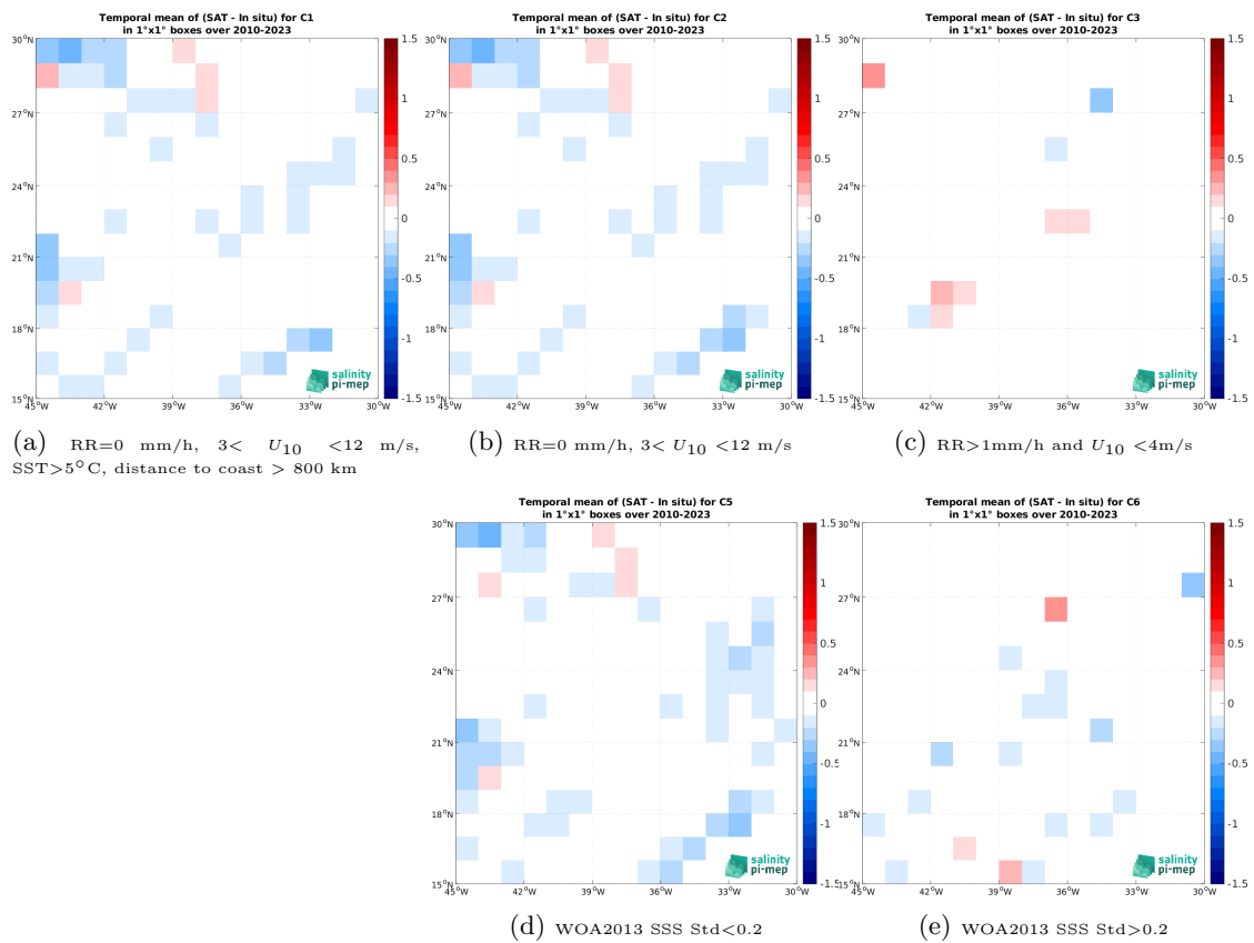
Figure 14: Temporal mean gridded over spatial boxes of size 1^\circ \times 1^\circ of \Delta SSS (SMOS SSS L4 v1 - Monthly (CMEMS-CNR) - TSG (LEGOS-DM)) for 5 different subdatasets corresponding to:RR=0 mm/h, 3 < U_{10} < 12 m/s, SST>5°C, distance to coast > 800 km (a), RR=0 mm/h, 3 < U_{10} < 12 m/s (b), RR>1mm/h and U_{10} < 4 m/s (c), WOA2013 SSS Std<0.2 (d), WOA2013 SSS Std>0.2 (e).
