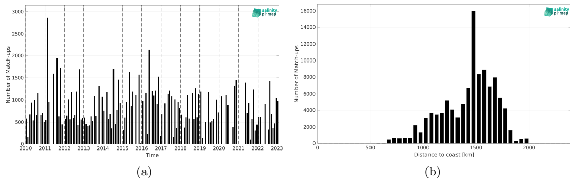
Figure 2: Number of match-ups between TSG (LEGOS-DM) and SMOS SSS L4 v1 - Monthly (CMEMS-CNR) SSS as a function of time (a) and as function of the distance to coast (b) over the SPURS 1 Pi-MEP region and for the full satellite product period.
