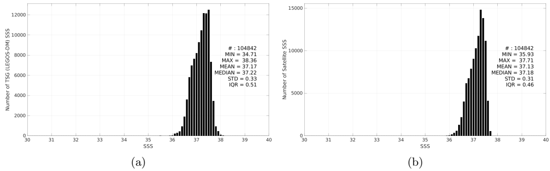
Figure 3: Histograms of SSS from TSG (LEGOS-DM) (a) and SMOS SSS L4 v1 - Monthly (CMEMS-CNR) (b) considering all match-up pairs per bins of 0.1 over the SPURS 1 Pi-MEP region and for the full satellite product period.
