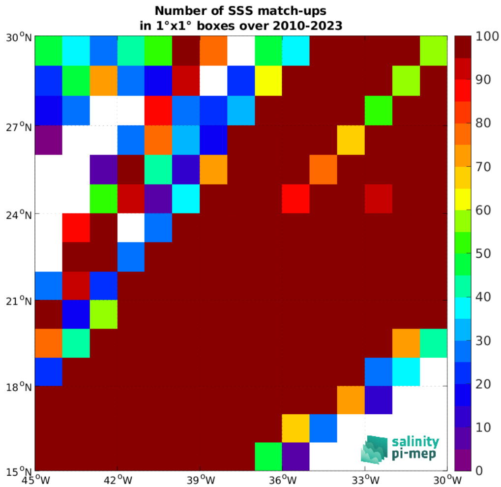
Figure 5: Number of SSS match-ups between TSG (LEGOS-DM) SSS and the SMOS SSS L4 v1 - Monthly (CMEMS-CNR) SSS product for the SPURS 1 Pi-MEP region over 1°x1° boxes and for the full satellite product period.
