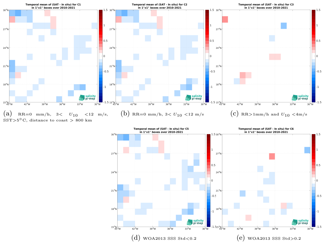
Figure 14: Temporal mean gridded over spatial boxes of size 1^\circ \times 1^\circ of \Delta SSS (SMOS SSS L4 v1 - Monthly (CMEMS-CNR) - TSG (LEGOS-DM)) for 5 different subdatasets corresponding to: RR=0 mm/h, 3 < U_{10} < 12 m/s, SST > 5^\circ C , distance to coast > 800 km (a), RR=0 mm/h, 3 < U_{10} < 12 m/s (b), RR > 1 mm/h and U_{10} < 4 m/s (c), WOA2013 SSS Std <0.2 (d), WOA2013 SSS Std >0.2 (e).
