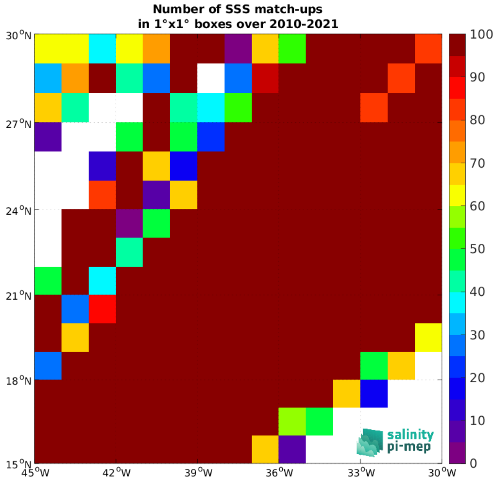
Figure 4: Number of SSS match-ups between TSG (LEGOS-DM) SSS and the SMOS SSS L4 v1 - Monthly (CMEMS-CNR) SSS product for the SPURS 1 Pi-MEP region over 1^\circ \times 1^\circ boxes and for the full satellite product period.
