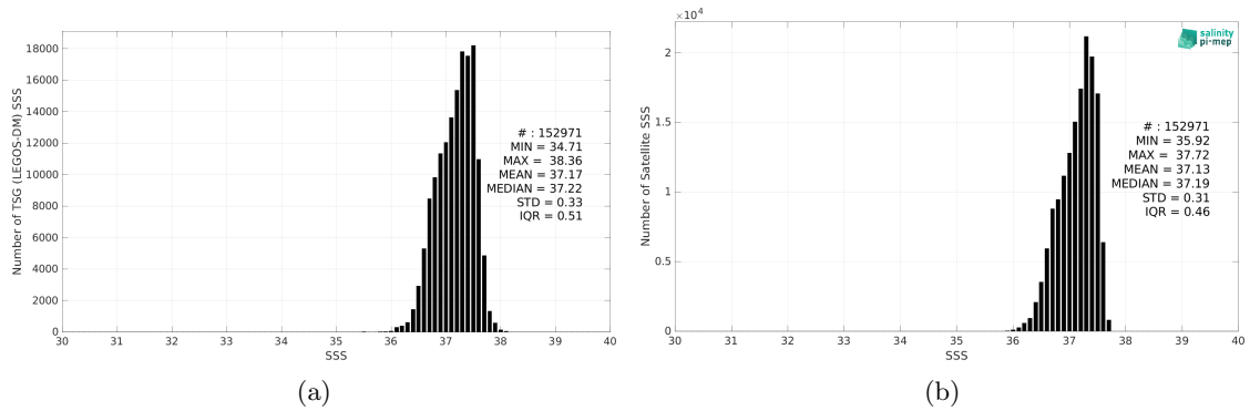
Figure 2: Histograms of SSS from TSG (LEGOS-DM) (a) and SMOS SSS L4 v1 - Monthly (CMEMS-CNR) (b) considering all match-up pairs per bins of 0.1 over the SPURS 1 Pi-MEP region and for the full satellite product period.
