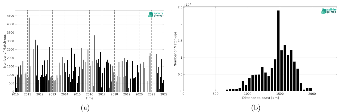
Figure 1: Number of match-ups between TSG (LEGOS-DM) and SMOS SSS L4 v1 - Monthly (CMEMS-CNR) SSS as a function of time (a) and as function of the distance to coast (b) over the SPURS 1 Pi-MEP region and for the full satellite product period.
