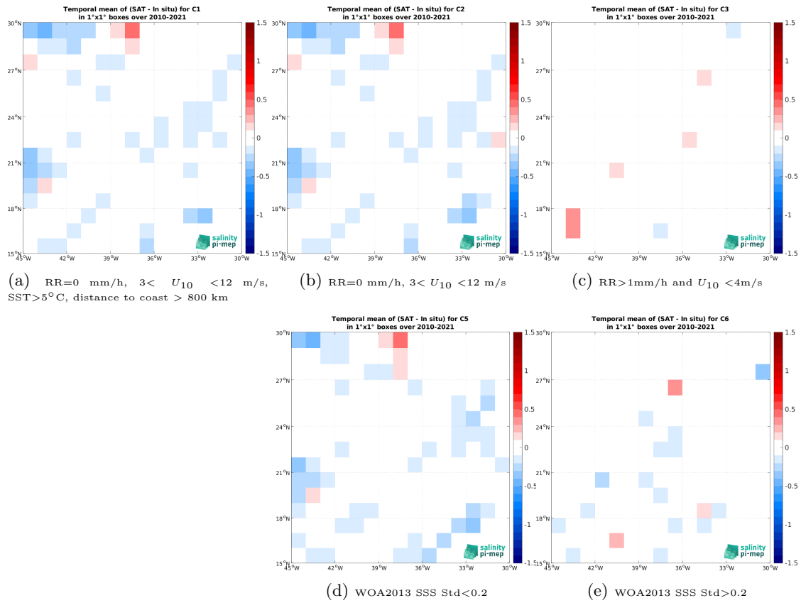
Figure 12: Temporal mean gridded over spatial boxes of size 1^\circ \times 1^\circ of \Delta\text{SSS} (SMOS SSS L4 v1 - Monthly (CMEMS-CNR) - TSG (LEGOS-DM)) for 5 different subdatasets corresponding to:RR=0 mm/h, 3 < U_{10} < 12 m/s, SST >5^\circ\text{C} , distance to coast > 800 km (a), RR=0 mm/h, 3 < U_{10} < 12 m/s (b), RR >1 mm/h and U_{10} < 4 m/s (c), WOA2013 SSS Std <0.2 (d), WOA2013 SSS Std >0.2 (e).
