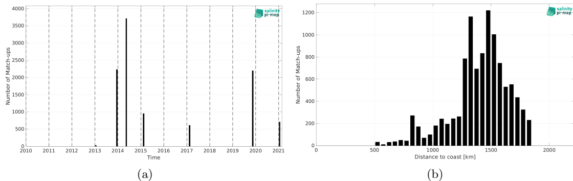
Figure 2: Number of match-ups between TSG (GOSUD-Sailing-ship) and SMOS SSS L4 v1 - Monthly (CMEMS-CNR) SSS as a function of time (a) and as function of the distance to coast (b) over the SPURS 1 Pi-MEP region and for the full satellite product period.
