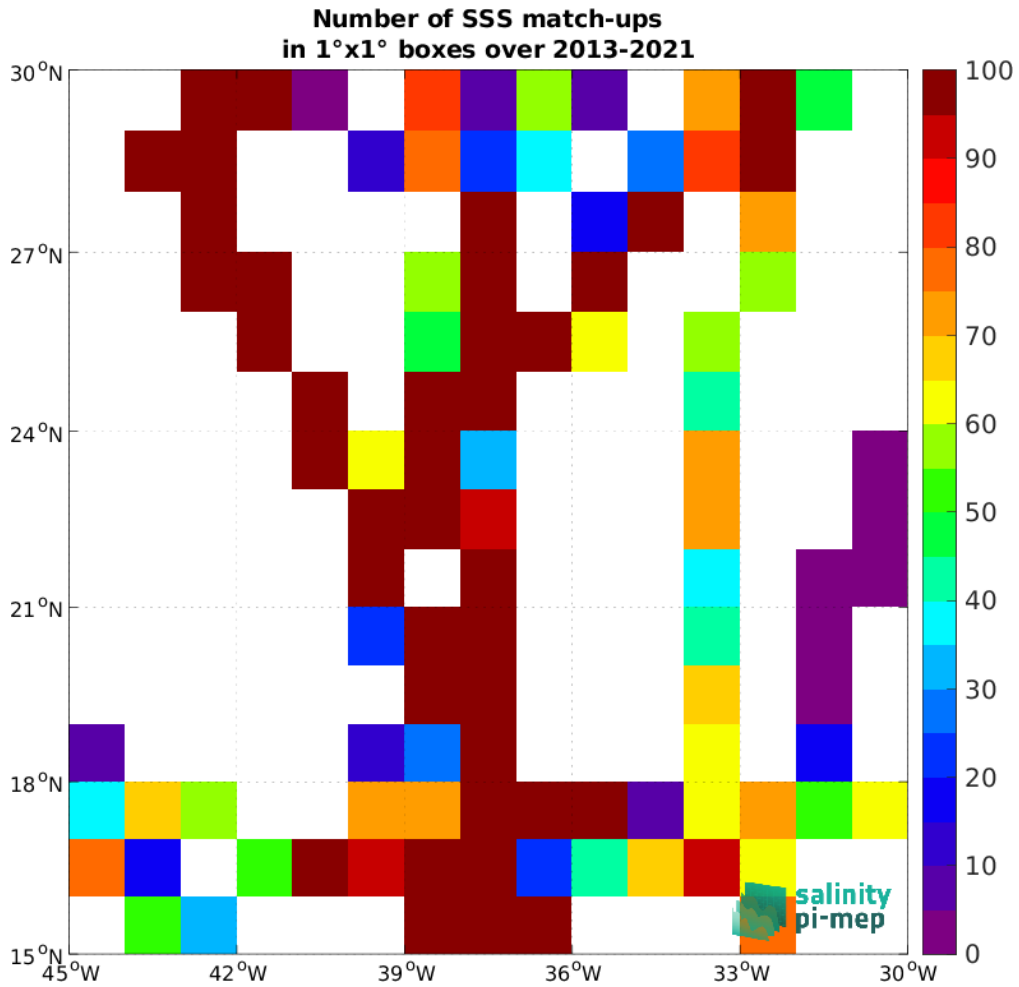
Figure 5: Number of SSS match-ups between TSG (GOSUD-Sailing-ship) SSS and the SMOS SSS L4 v1 - Monthly (CMEMS-CNR) SSS product for the SPURS 1 Pi-MEP region over 1^\circ \times 1^\circ boxes and for the full satellite product period.
