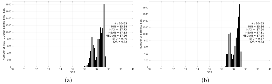
Figure 3: Histograms of SSS from TSG (GOSUD-Sailing-ship) (a) and SMOS SSS L4 v1 - Monthly (CMEMS-CNR) (b) considering all match-up pairs per bins of 0.1 over the SPURS 1 Pi-MEP region and for the full satellite product period.
