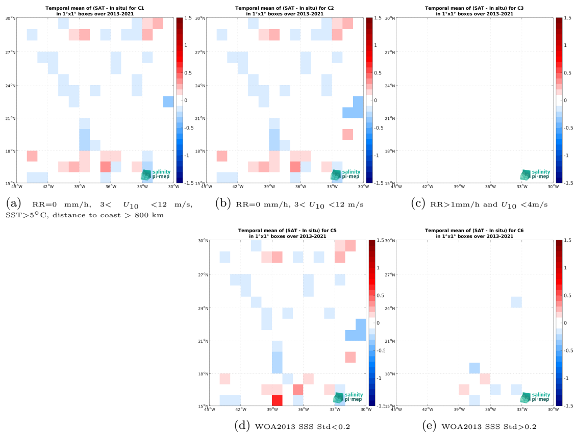
Figure 14: Temporal mean gridded over spatial boxes of size 1^\circ \times 1^\circ of \Delta SSS (SMOS SSS L4 v1 - Monthly (CMEMS-CNR) - TSG (GOSUD-Sailing-ship)) for 5 different subdatasets corresponding to: RR=0 mm/h, 3 < U_{10} < 12 m/s, SST > 5^\circ C , distance to coast > 800 km (a), RR=0 mm/h, 3 < U_{10} < 12 m/s (b), RR > 1 mm/h and U_{10} < 4 m/s (c), WOA2013 SSS Std < 0.2 (d), WOA2013 SSS Std > 0.2 (e).
