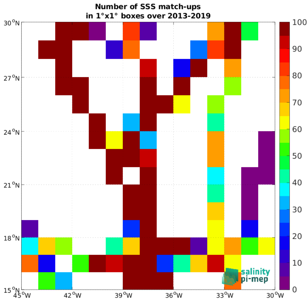
Figure 5: Number of SSS match-ups between TSG (GOSUD-Sailing-ship) SSS and the SMOS SSS L4 v1 - Monthly (CMEMS-CNR) SSS product for the SPURS 1 Pi-MEP region over 1°x1° boxes and for the full satellite product period.
