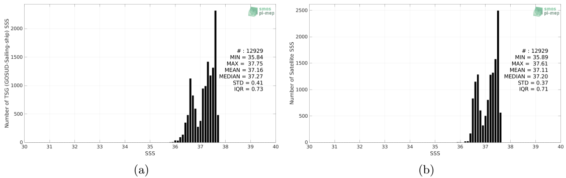
Figure 2: Histograms of SSS from TSG (GOSUD-Sailing-ship) (a) and SMOS SSS L4 v1 - Monthly (CMEMS-CNR) (b) considering all match-up pairs per bins of 0.1 over the SPURS 1 Pi-MEP region and for the full satellite product period.
