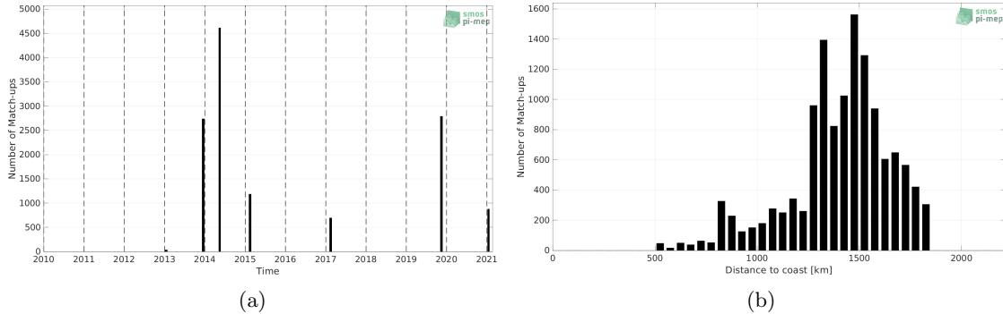
Figure 1: Number of match-ups between TSG (GOSUD-Sailing-ship) and SMOS SSS L4 v1 - Monthly (CMEMS-CNR) SSS as a function of time (a) and as function of the distance to coast (b) over the SPURS 1 Pi-MEP region and for the full satellite product period.
