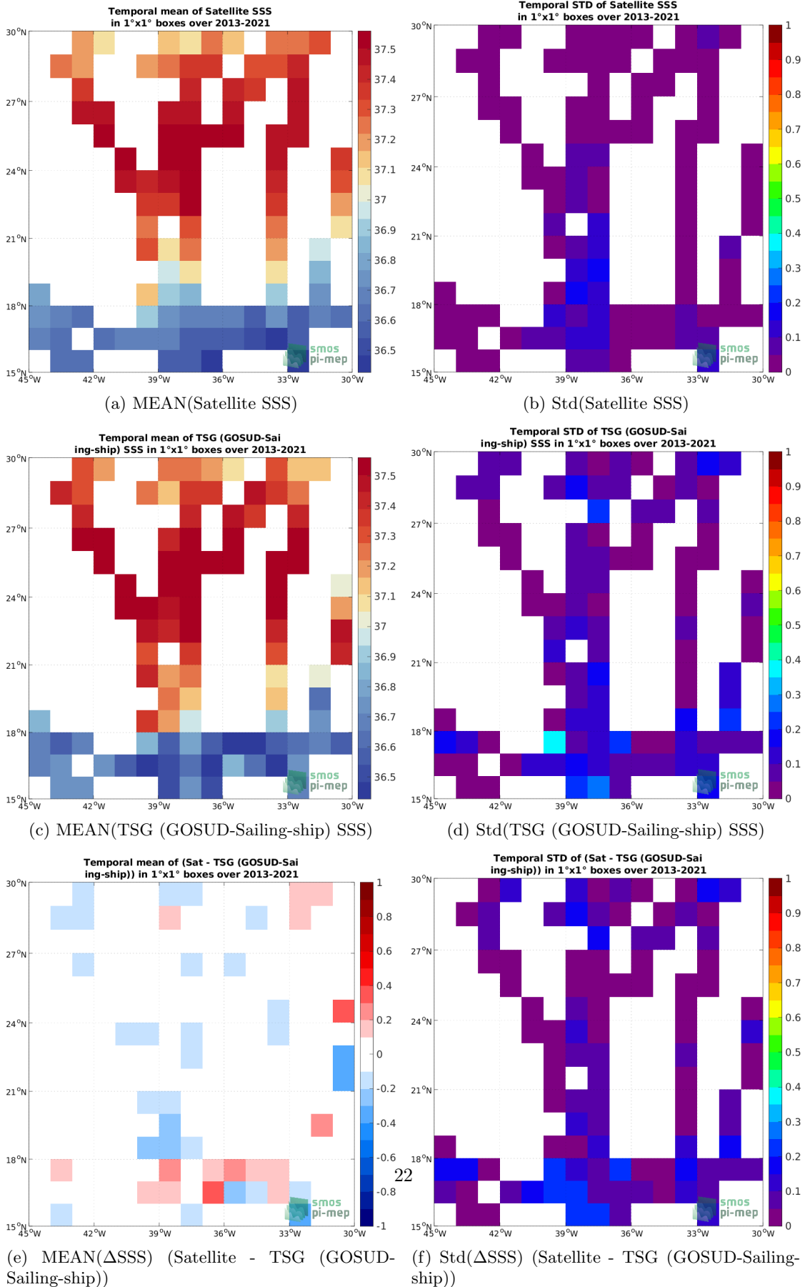
Figure 6: Temporal mean (left) and Std (right) of SSS from SMOS SSS L4 v1 - Monthly (CMEMS-CNR) (top), TSG (GOSUD-Sailing-ship) (middle), and of \Delta SSS (Satellite - TSG (GOSUD-Sailing-ship)). Only match-up pairs are used to generate these maps.
