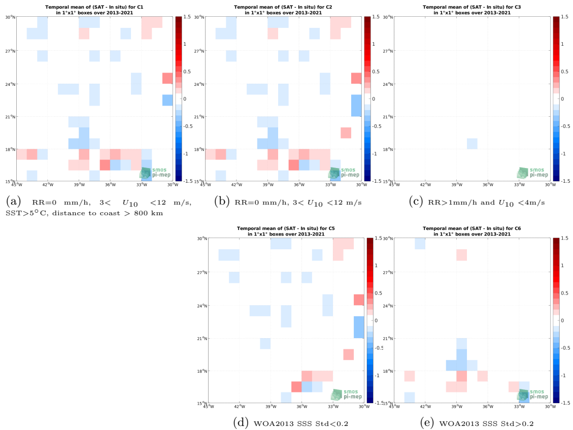
Figure 12: Temporal mean gridded over spatial boxes of size 1^\circ \times 1^\circ of \Delta SSS (SMOS SSS L4 v1 - Monthly (CMEMS-CNR) - TSG (GOSUD-Sailing-ship)) for 5 different subdatasets corresponding to:RR=0 mm/h, 3 < U_{10} < 12 m/s, SST >5^\circ C, distance to coast > 800 km (a), RR=0 mm/h, 3 < U_{10} < 12 m/s (b), RR >1 mm/h and U_{10} < 4 m/s (c), WOA2013 SSS Std <0.2 (d), WOA2013 SSS Std >0.2 (e).
