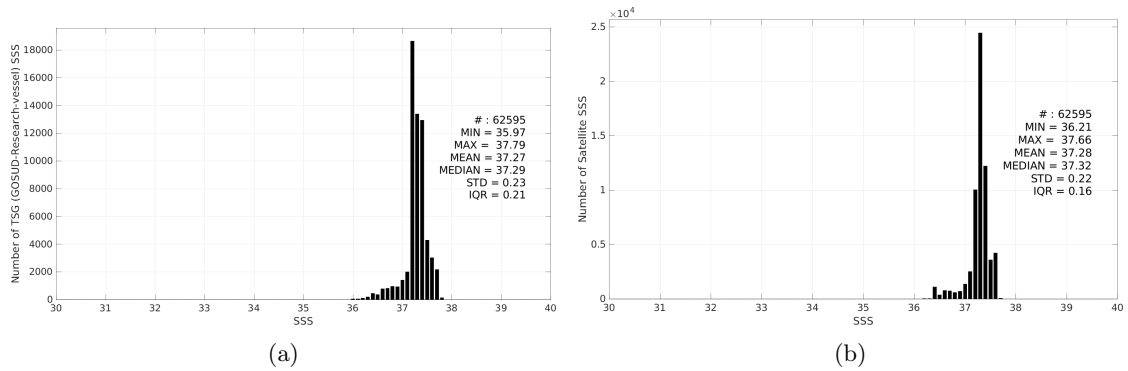
Figure 3: Histograms of SSS from TSG (GOSUD-Research-vessel) (a) and SMOS SSS L4 v1 - Monthly (CMEMS-CNR) (b) considering all match-up pairs per bins of 0.1 over the SPURS 1 Pi-MEP region and for the full satellite product period.
