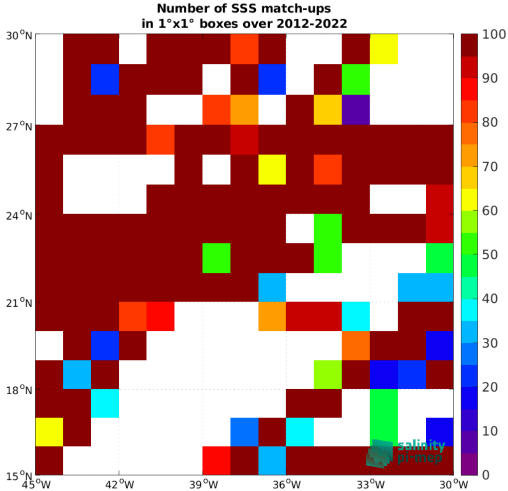
Figure 5: Number of SSS match-ups between TSG (GOSUD-Research-vessel) SSS and the SMOS SSS L4 v1 - Monthly (CMEMS-CNR) SSS product for the SPURS 1 Pi-MEP region over 1^\circ \times 1^\circ boxes and for the full satellite product period.
