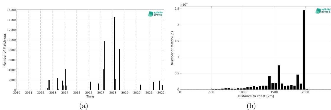
Figure 2: Number of match-ups between TSG (GOSUD-Research-vessel) and SMOS SSS L4 v1 - Monthly (CMEMS-CNR) SSS as a function of time (a) and as function of the distance to coast (b) over the SPURS 1 Pi-MEP region and for the full satellite product period.
