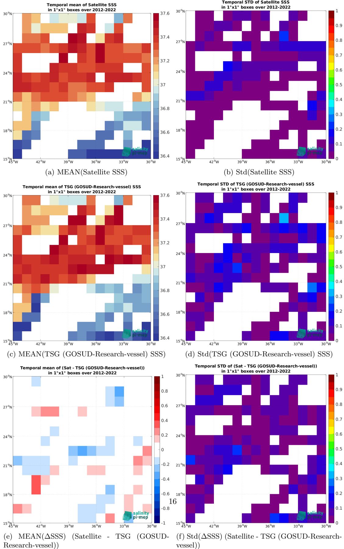
Figure 7: Temporal mean (left) and Std (right) of SSS from SMOS SSS L4 v1 - Monthly (CMEMS-CNR) (top), TSG (GOSUD-Research-vessel) (middle), and of \Delta SSS (Satellite - TSG (GOSUD-Research-vessel)). Only match-up pairs are used to generate these maps.
