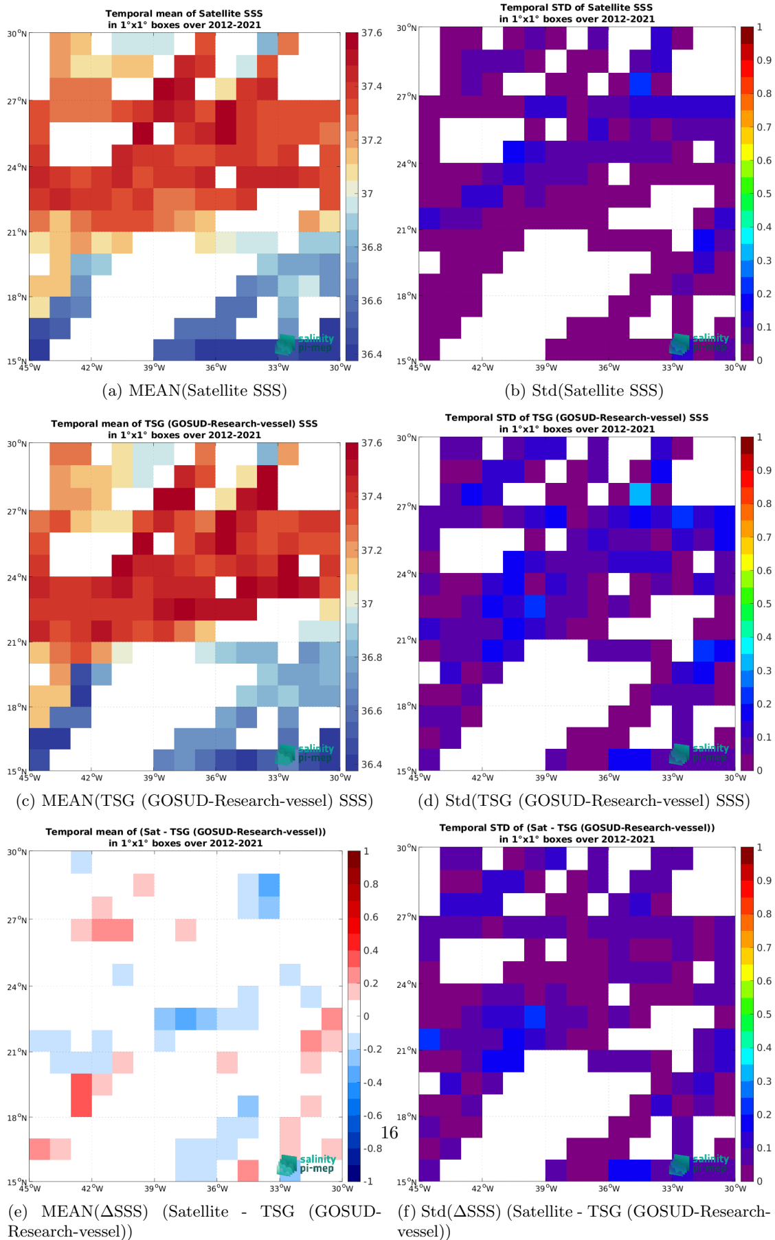
Figure 6: Temporal mean (left) and Std (right) of SSS from SMOS SSS L4 v1 - Monthly (CMEMS-CNR) (top), TSG (GOSUD-Research-vessel) (middle), and of \Delta SSS (Satellite - TSG (GOSUD-Research-vessel)). Only match-up pairs are used to generate these maps.
