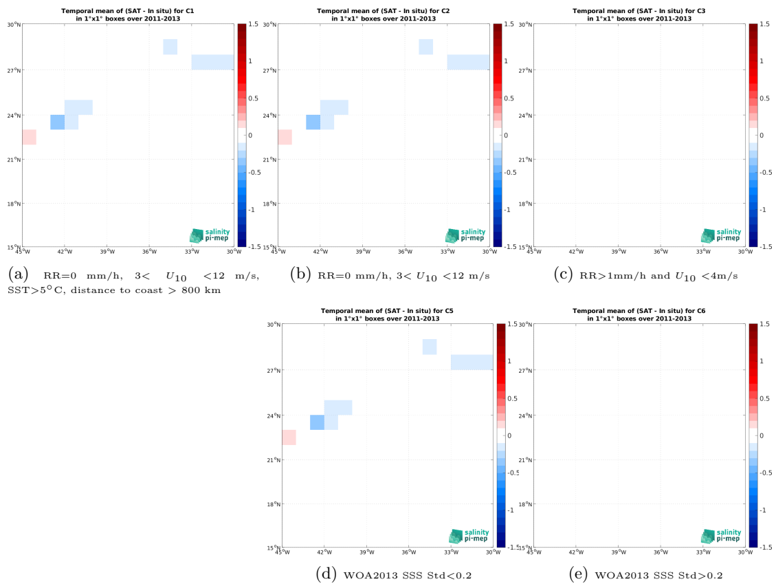
Figure 14: Temporal mean gridded over spatial boxes of size 1^\circ \times 1^\circ of \Delta SSS (SMOS SSS L4 v1 - Monthly (CMEMS-CNR) - TSG (CSIC-UTM)) for 5 different subdatasets corresponding to:RR=0 mm/h, 3 < U_{10} < 12 m/s, SST >5^\circ C, distance to coast > 800 km (a), RR=0 mm/h, 3 < U_{10} < 12 m/s (b), RR >1 mm/h and U_{10} < 4 m/s (c), WOA2013 SSS Std <0.2 (d), WOA2013 SSS Std >0.2 (e).
