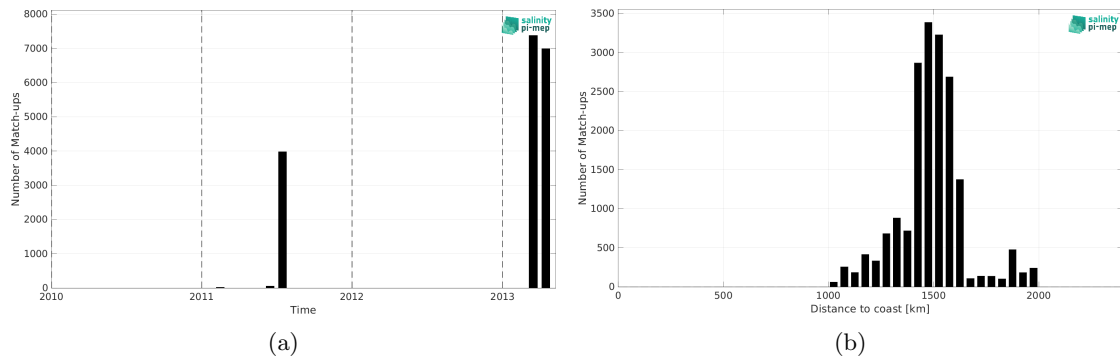
Figure 2: Number of match-ups between TSG (CSIC-UTM) and SMOS SSS L4 v1 - Monthly (CMEMS-CNR) SSS as a function of time (a) and as function of the distance to coast (b) over the SPURS 1 Pi-MEP region and for the full satellite product period.
