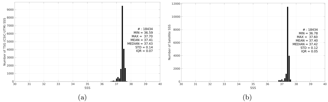
Figure 3: Histograms of SSS from TSG (CSIC-UTM) (a) and SMOS SSS L4 v1 - Monthly (CMEMS-CNR) (b) considering all match-up pairs per bins of 0.1 over the SPURS 1 Pi-MEP region and for the full satellite product period.
