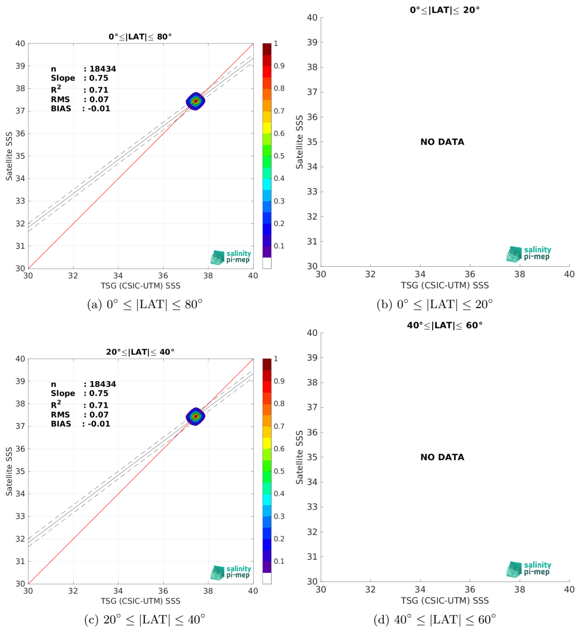
Figure 10: Contour maps of the concentration of SMOS SSS L4 v1 - Monthly (CMEMS-CNR) SSS (y-axis) versus TSG (CSIC-UTM) SSS (x-axis) at match-up pairs for different latitude bands. For each plot, the red line shows x=y . The black thin and dashed lines indicate a linear fit through the data cloud and the \pm 95\% confidence levels, respectively. The number match-up pairs n , the slope and R^2 coefficient of the linear fit, the root mean square (RMS) and the mean bias between satellite and in situ data are indicated for each latitude band in each plots.
