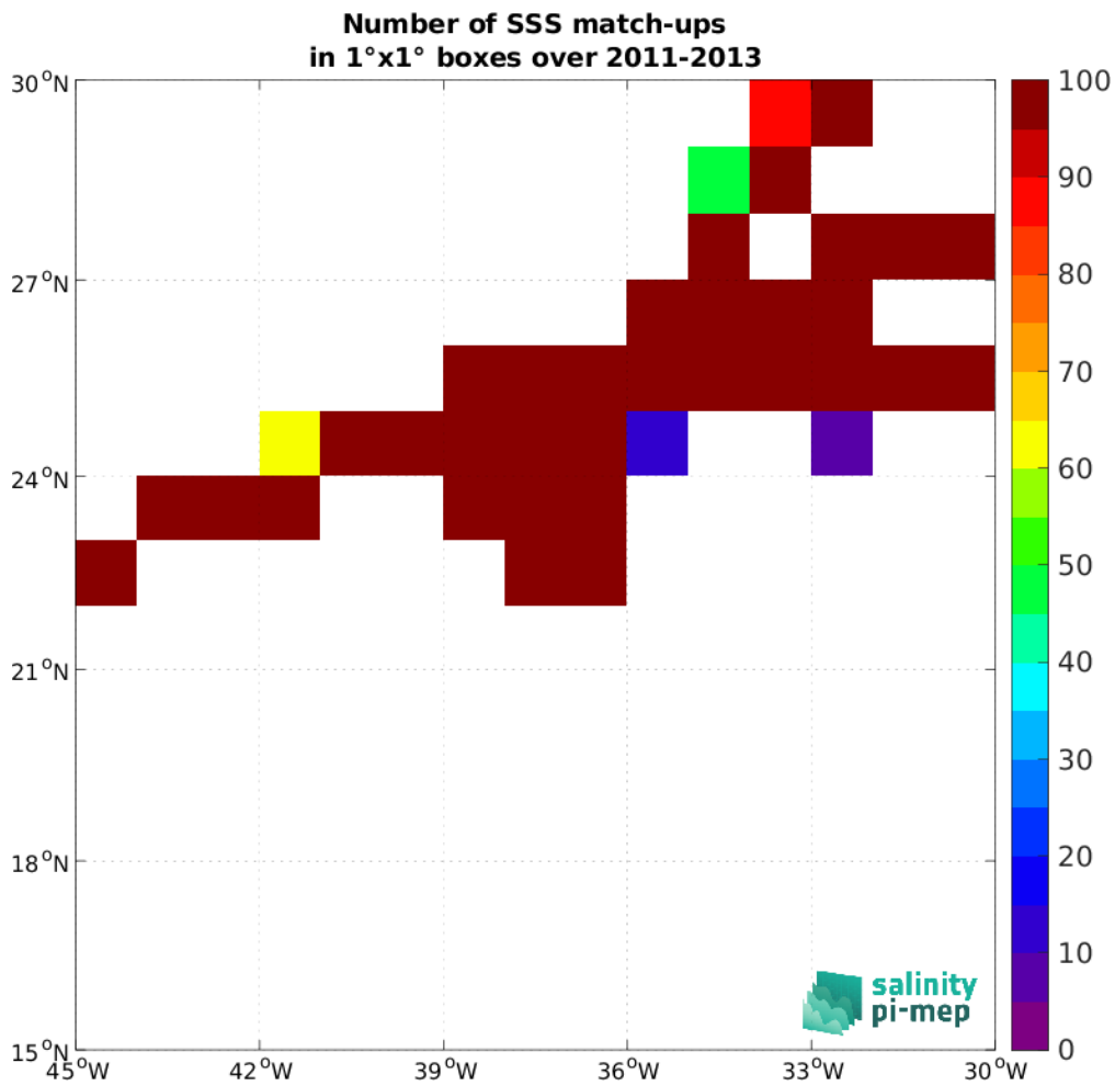
Figure 5: Number of SSS match-ups between TSG (CSIC-UTM) SSS and the SMOS SSS L4 v1 - Monthly (CMEMS-CNR) SSS product for the SPURS 1 Pi-MEP region over 1^\circ \times 1^\circ boxes and for the full satellite product period.
