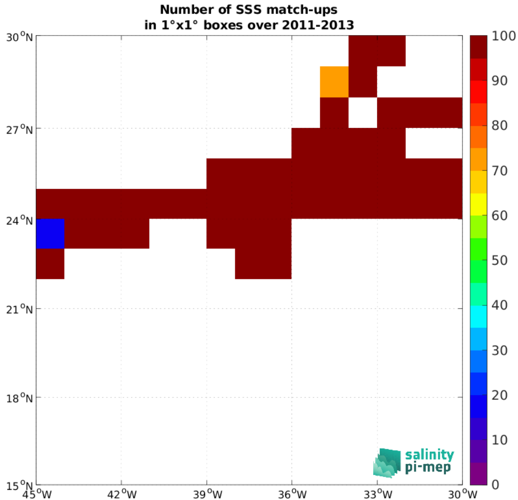
Figure 4: Number of SSS match-ups between TSG (CSIC-UTM) SSS and the SMOS SSS L4 v1 - Monthly (CMEMS-CNR) SSS product for the SPURS 1 Pi-MEP region over 1^\circ \times 1^\circ boxes and for the full satellite product period.
