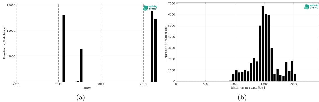
Figure 1: Number of match-ups between TSG (CSIC-UTM) and SMOS SSS L4 v1 - Monthly (CMEMS-CNR) SSS as a function of time (a) and as function of the distance to coast (b) over the SPURS 1 Pi-MEP region and for the full satellite product period.
