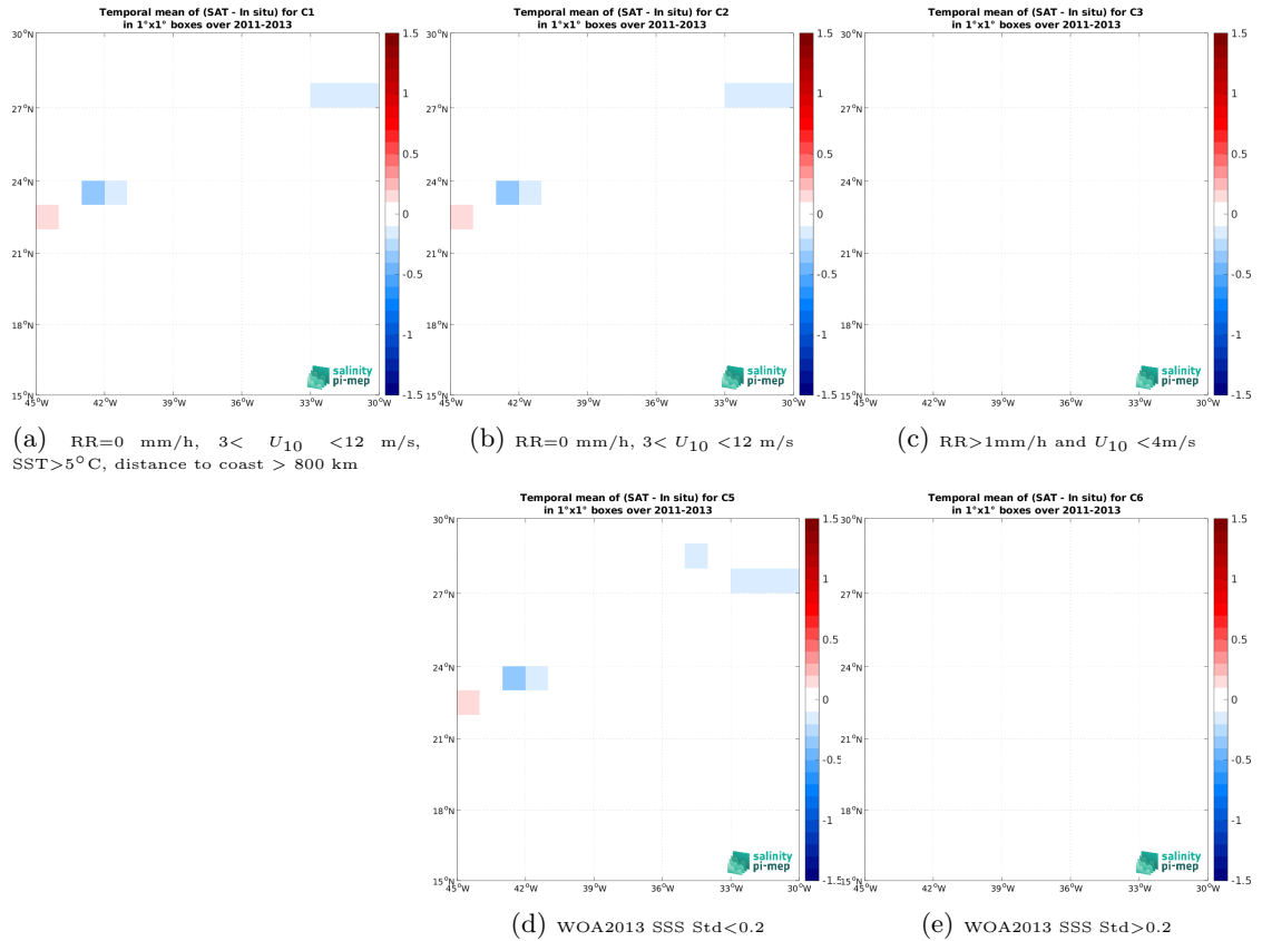
Figure 12: Temporal mean gridded over spatial boxes of size 1^{\circ}\times 1^{\circ} of \Delta\text{SSS} (SMOS SSS L4 v1 - Monthly (CMEMS-CNR) - TSG (CSIC-UTM)) for 5 different subdatasets corresponding to:RR=0 mm/h, 3 < U_{10} < 12 m/s, SST >5^{\circ}\text{C} , distance to coast > 800 km (a), RR=0 mm/h, 3 < U_{10} < 12 m/s (b), RR >1\text{mm/h} and U_{10} < 4\text{m/s} (c), WOA2013 SSS Std <0.2 (d), WOA2013 SSS Std >0.2 (e).
