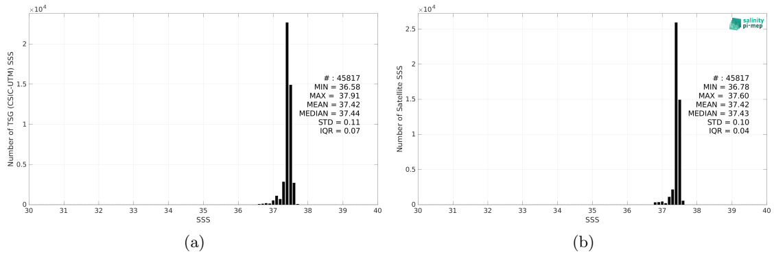
Figure 2: Histograms of SSS from TSG (CSIC-UTM) (a) and SMOS SSS L4 v1 - Monthly (CMEMS-CNR) (b) considering all match-up pairs per bins of 0.1 over the SPURS 1 Pi-MEP region and for the full satellite product period.
