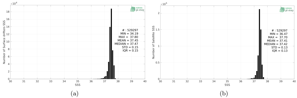
Figure 2: Histograms of SSS from Surface drifters (a) and SMOS SSS L4 v1 - Monthly (CMEMS-CNR) (b) considering all match-up pairs per bins of 0.1 over the SPURS 1 Pi-MEP region and for the full satellite product period.
