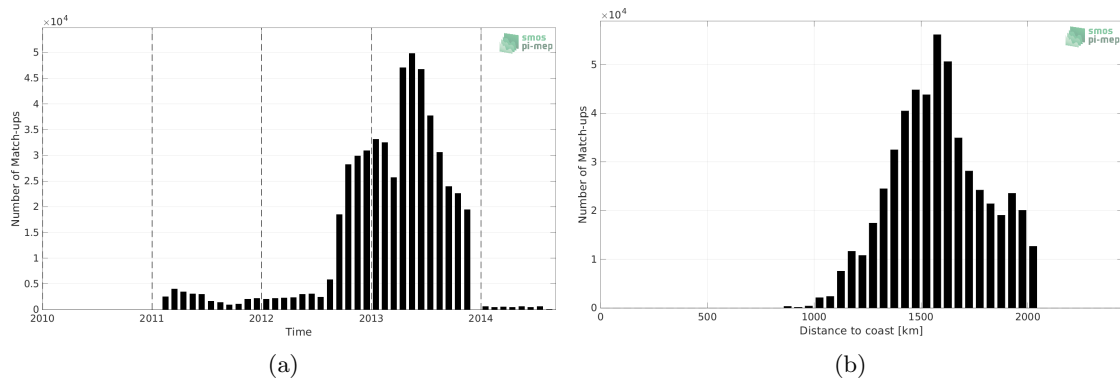
Figure 1: Number of match-ups between Surface drifters and SMOS SSS L4 v1 - Monthly (CMEMS-CNR) SSS as a function of time (a) and as function of the distance to coast (b) over the SPURS 1 Pi-MEP region and for the full satellite product period.
