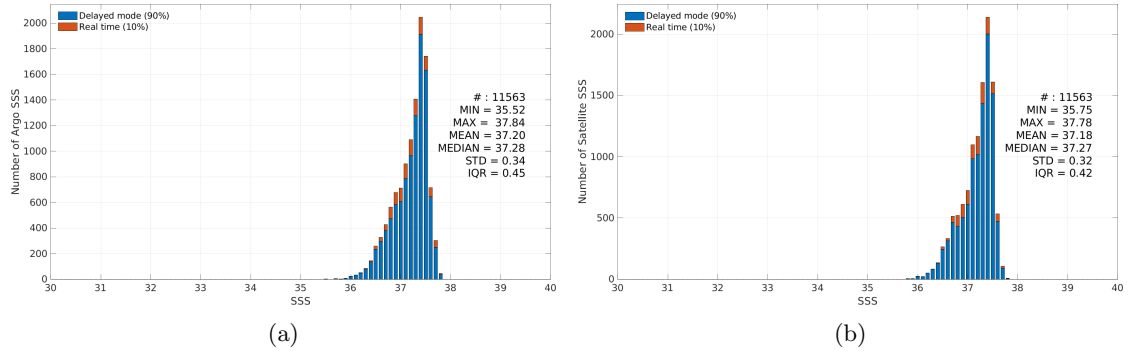
Figure 3: Histograms of SSS from Argo (a) and SMOS SSS L4 v1 - Monthly (CMEMS-CNR) (b) considering all match-up pairs per bins of 0.1 over the SPURS 1 Pi-MEP region and for the full satellite product period.
