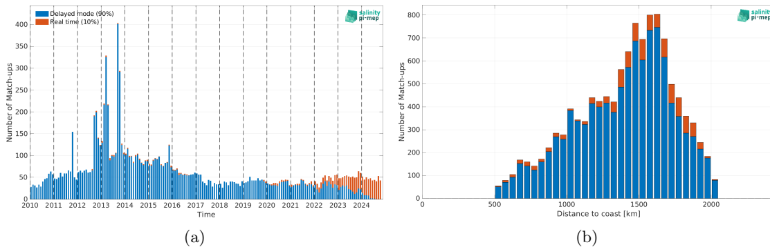
Figure 2: Number of match-ups between Argo and SMOS SSS L4 v1 - Monthly (CMEMS-CNR) SSS as a function of time (a) and as function of the distance to coast (b) over the SPURS 1 Pi-MEP region and for the full satellite product period.
