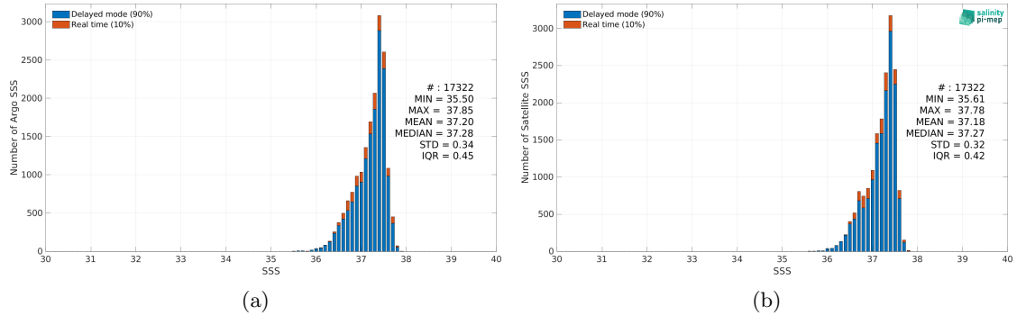
Figure 2: Histograms of SSS from Argo (a) and SMOS SSS L4 v1 - Monthly (CMEMS-CNR) (b) considering all match-up pairs per bins of 0.1 over the SPURS 1 Pi-MEP region and for the full satellite product period.
