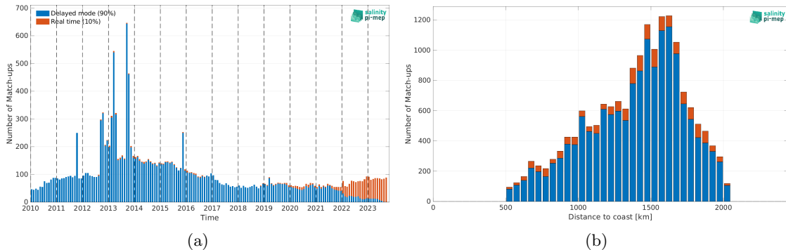
Figure 1: Number of match-ups between Argo and SMOS SSS L4 v1 - Monthly (CMEMS-CNR) SSS as a function of time (a) and as function of the distance to coast (b) over the SPURS 1 Pi-MEP region and for the full satellite product period.
