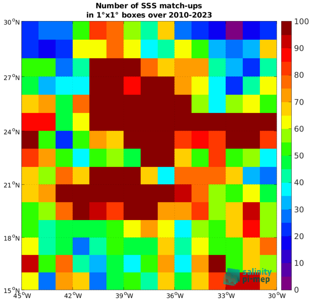
Figure 4: Number of SSS match-ups between Argo SSS and the SMOS SSS L4 v1 - Monthly (CMEMS-CNR) SSS product for the SPURS 1 Pi-MEP region over 1^\circ \times 1^\circ boxes and for the full satellite product period.
