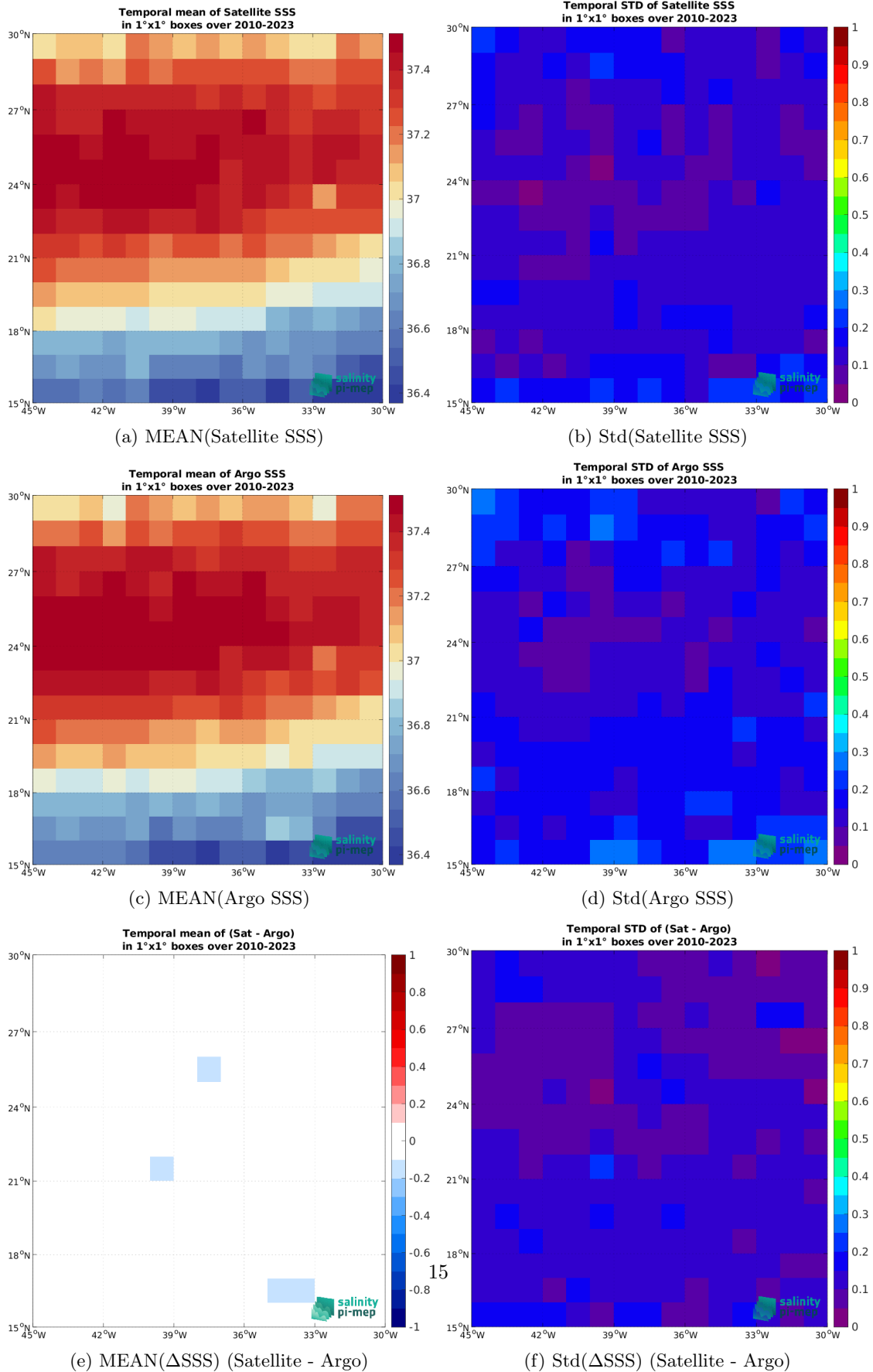
Figure 6: Temporal mean (left) and Std (right) of SSS from SMOS SSS L4 v1 - Monthly (CMEMS-CNR) (top), Argo (middle), and of \Delta SSS (Satellite - Argo). Only match-up pairs are used to generate these maps.
