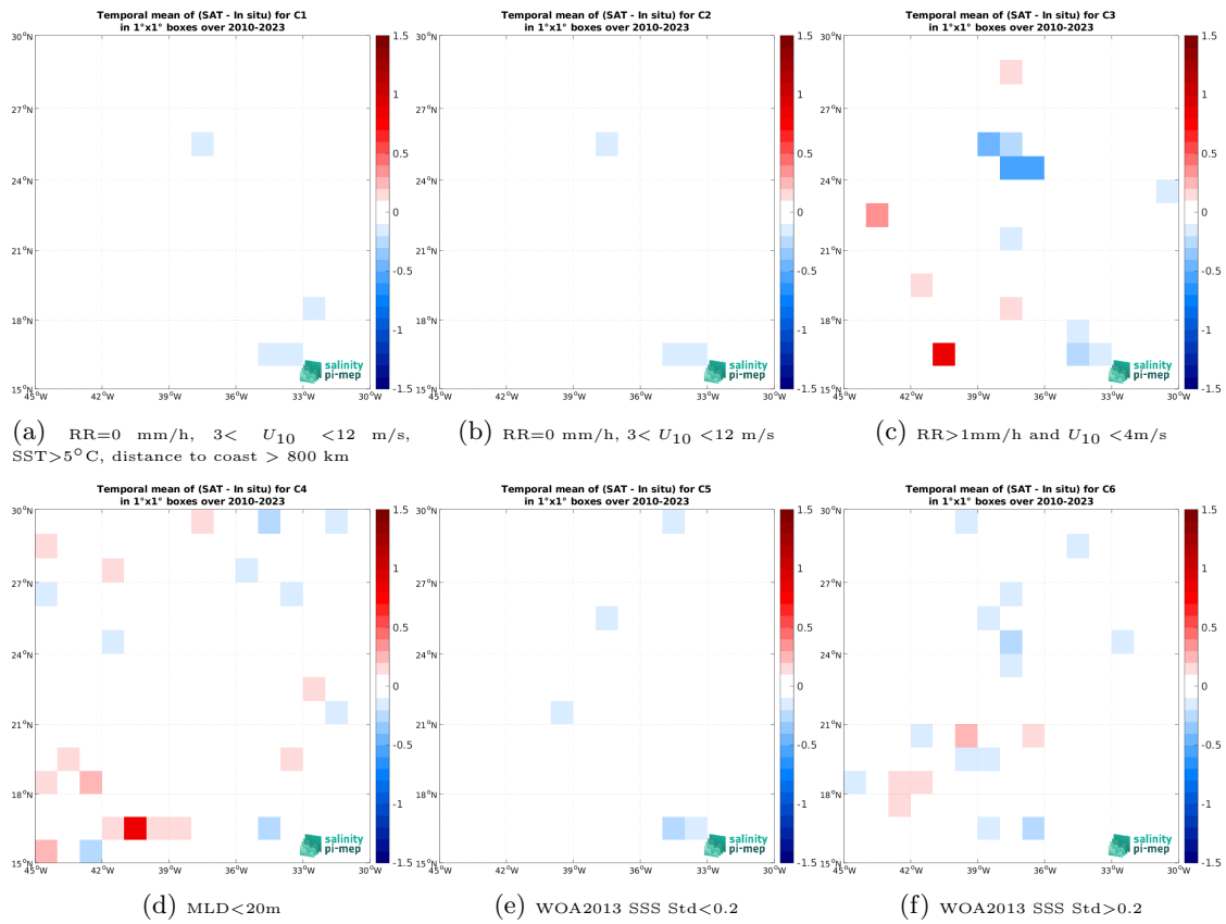
Figure 12: Temporal mean gridded over spatial boxes of size 1^\circ \times 1^\circ of \Delta SSS (SMOS SSS L4 v1 - Monthly (CMEMS-CNR) - Argo) for 6 different subdatasets corresponding to:RR=0 mm/h, 3 < U_{10} < 12 m/s, SST >5^\circ\text{C} , distance to coast > 800 km (a), RR=0 mm/h, 3 < U_{10} < 12 m/s (b), RR >1 mm/h and U_{10} < 4 m/s (c),MLD <20 m (d),WOA2013 SSS Std <0.2 (e),WOA2013 SSS Std >0.2 (f).
