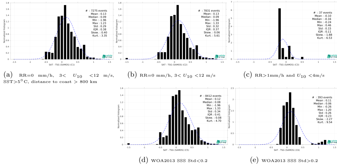
Figure 15: Normalized histogram of \Delta\text{SSS} (SMOS SSS L4 v1 - Daily (CMEMS-CNR) - TSG (SAMOS)) for 5 different subdatasets corresponding to: RR=0 mm/h, 3 < U_{10} < 12 m/s, SST > 5^\circ\text{C} , distance to coast > 800 km (a), RR=0 mm/h, 3 < U_{10} < 12 m/s (b), RR > 1\text{mm/h} and U_{10} < 4\text{m/s} (c), WOA2013 SSS Std < 0.2 (d), WOA2013 SSS Std > 0.2 (e).
