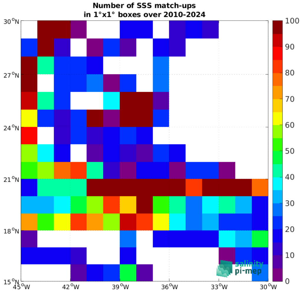
Figure 5: Number of SSS match-ups between TSG (SAMOS) SSS and the SMOS SSS L4 v1 - Daily (CMEMS-CNR) SSS product for the SPURS 1 Pi-MEP region over 1^\circ \times 1^\circ boxes and for the full satellite product period.
