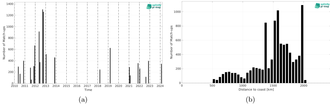
Figure 2: Number of match-ups between TSG (SAMOS) and SMOS SSS L4 v1 - Daily (CMEMS-CNR) SSS as a function of time (a) and as function of the distance to coast (b) over the SPURS 1 Pi-MEP region and for the full satellite product period.
