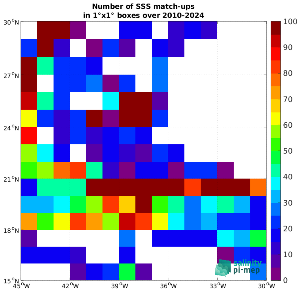
Figure 5: Number of SSS match-ups between TSG (SAMOS) SSS and the SMOS SSS L4 v1 - Daily (CMEMS-CNR) SSS product for the SPURS 1 Pi-MEP region over 1°x1° boxes and for the full satellite product period.
