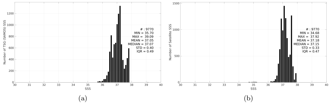
Figure 3: Histograms of SSS from TSG (SAMOS) (a) and SMOS SSS L4 v1 - Daily (CMEMS-CNR) (b) considering all match-up pairs per bins of 0.1 over the SPURS 1 Pi-MEP region and for the full satellite product period.
