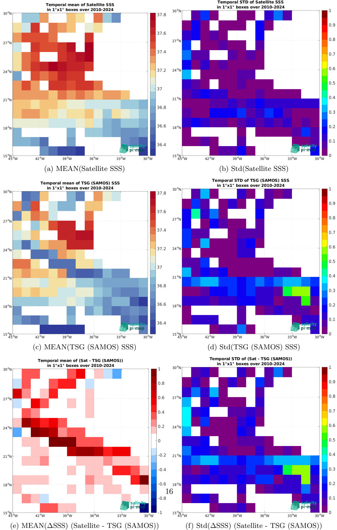
Figure 7: Temporal mean (left) and Std (right) of SSS from SMOS SSS L4 v1 - Daily (CMEMS-CNR) (top), TSG (SAMOS) (middle), and of \Delta SSS (Satellite - TSG (SAMOS)). Only match-up pairs are used to generate these maps.
