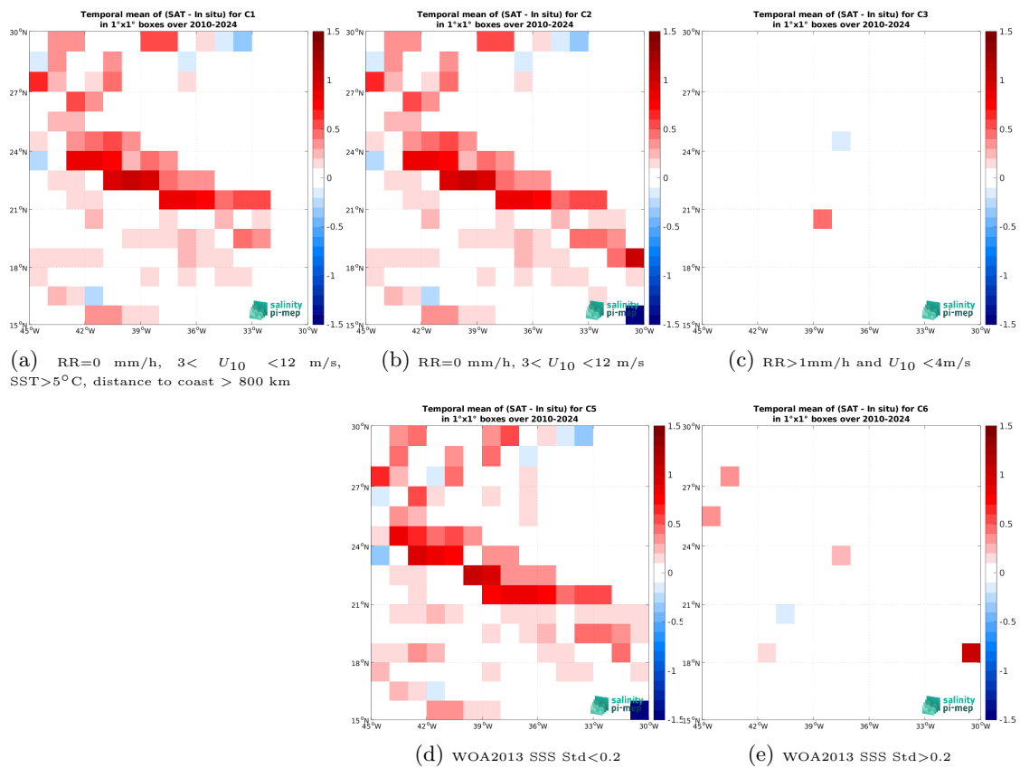
Figure 14: Temporal mean gridded over spatial boxes of size 1^\circ \times 1^\circ of \Delta SSS (SMOS SSS L4 v1 - Daily (CMEMS-CNR) - TSG (SAMOS)) for 5 different subdatasets corresponding to: RR=0 mm/h, 3 < U_{10} < 12 m/s, SST > 5^\circ C , distance to coast > 800 km (a), RR=0 mm/h, 3 < U_{10} < 12 m/s (b), RR > 1 mm/h and U_{10} < 4 m/s (c), WOA2013 SSS Std < 0.2 (d), WOA2013 SSS Std > 0.2 (e).
