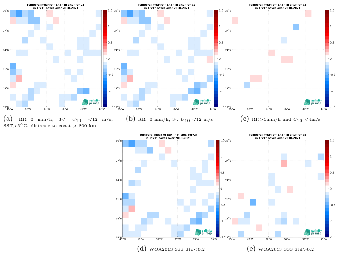
Figure 14: Temporal mean gridded over spatial boxes of size 1^\circ \times 1^\circ of \Delta SSS (SMOS SSS L4 v1 - Daily (CMEMS-CNR) - TSG (LEGOS-DM)) for 5 different subdatasets corresponding to: RR=0 mm/h, 3 < U_{10} < 12 m/s, SST > 5^\circ C , distance to coast > 800 km (a), RR=0 mm/h, 3 < U_{10} < 12 m/s (b), RR > 1 mm/h and U_{10} < 4 m/s (c), WOA2013 SSS Std < 0.2 (d), WOA2013 SSS Std > 0.2 (e).
