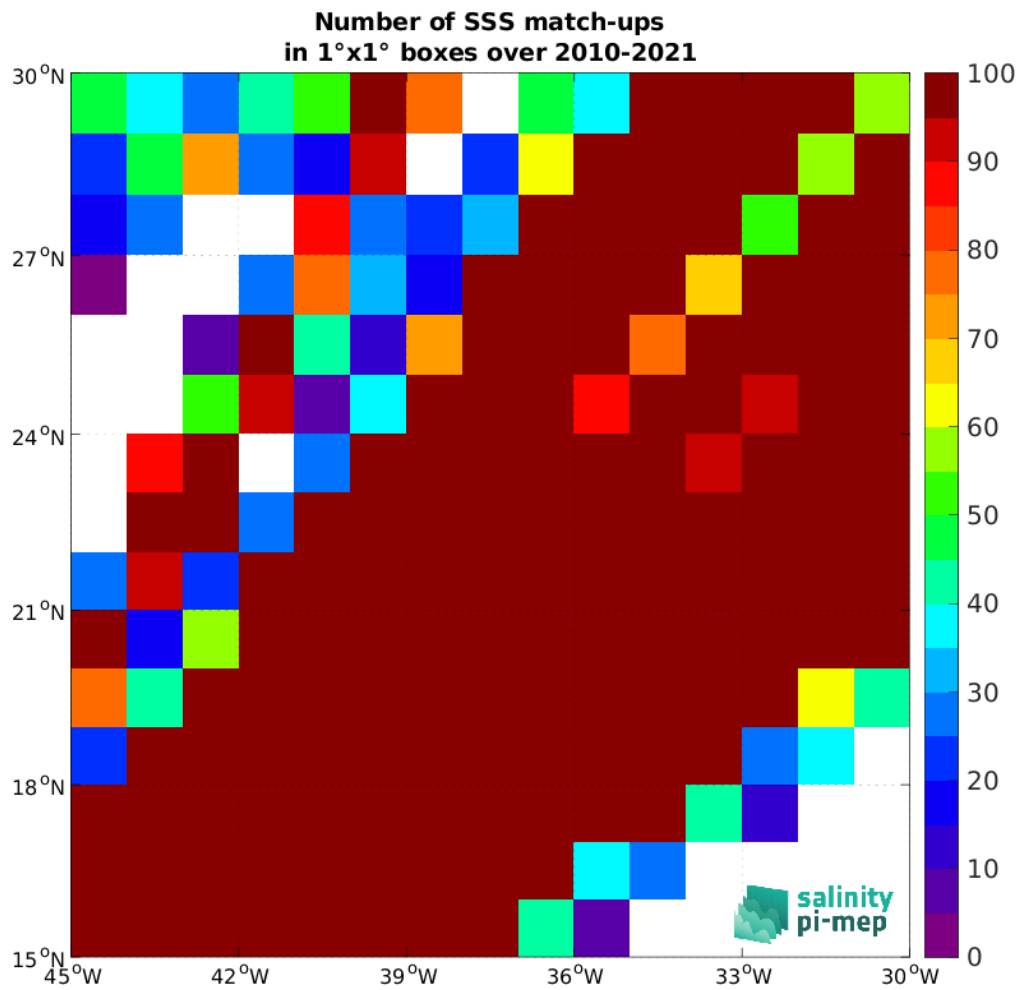
Figure 5: Number of SSS match-ups between TSG (LEGOS-DM) SSS and the SMOS SSS L4 v1 - Daily (CMEMS-CNR) SSS product for the SPURS 1 Pi-MEP region over 1^\circ \times 1^\circ boxes and for the full satellite product period.
