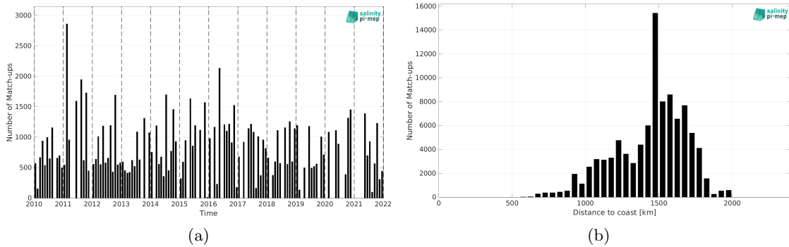
Figure 2: Number of match-ups between TSG (LEGOS-DM) and SMOS SSS L4 v1 - Daily (CMEMS-CNR) SSS as a function of time (a) and as function of the distance to coast (b) over the SPURS 1 Pi-MEP region and for the full satellite product period.
