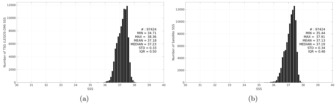
Figure 3: Histograms of SSS from TSG (LEGOS-DM) (a) and SMOS SSS L4 v1 - Daily (CMEMS-CNR) (b) considering all match-up pairs per bins of 0.1 over the SPURS 1 Pi-MEP region and for the full satellite product period.
