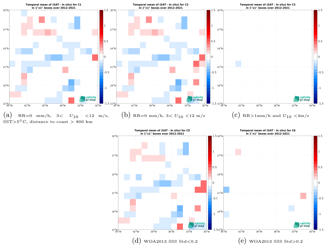
Figure 14: Temporal mean gridded over spatial boxes of size 1^\circ \times 1^\circ of \Delta\text{SSS} (SMOS SSS L4 v1 - Daily (CMEMS-CNR) - TSG (GOSUD-Research-vessel)) for 5 different subdatasets corresponding to:RR=0 mm/h, 3 < U_{10} < 12 m/s, SST>5°C, distance to coast > 800 km (a), RR=0 mm/h, 3 < U_{10} < 12 m/s (b), RR>1mm/h and U_{10} < 4 m/s (c), WOA2013 SSS Std<0.2 (d), WOA2013 SSS Std>0.2 (e).
