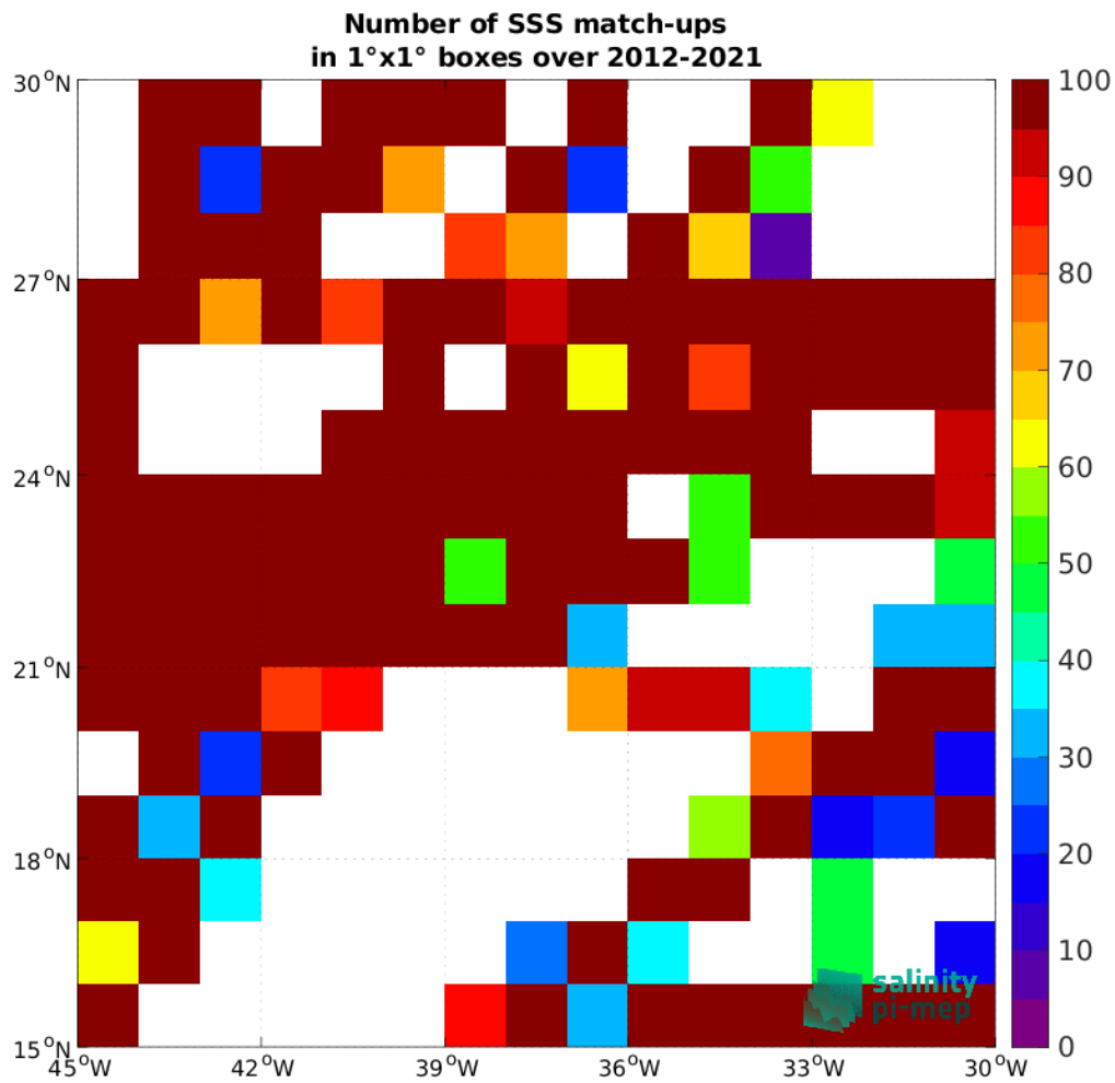
Figure 5: Number of SSS match-ups between TSG (GOSUD-Research-vessel) SSS and the SMOS SSS L4 v1 - Daily (CMEMS-CNR) SSS product for the SPURS 1 Pi-MEP region over 1°x1° boxes and for the full satellite product period.
