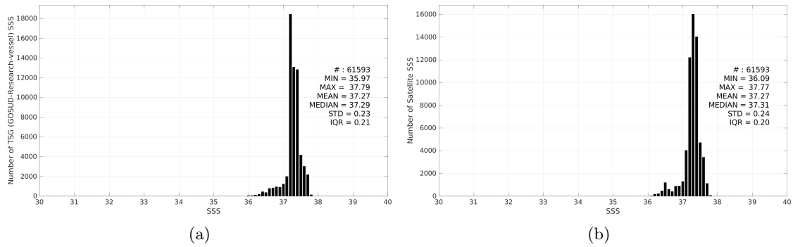
Figure 3: Histograms of SSS from TSG (GOSUD-Research-vessel) (a) and SMOS SSS L4 v1 - Daily (CMEMS-CNR) (b) considering all match-up pairs per bins of 0.1 over the SPURS 1 Pi-MEP region and for the full satellite product period.
