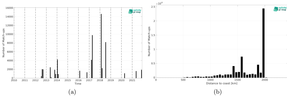
Figure 2: Number of match-ups between TSG (GOSUD-Research-vessel) and SMOS SSS L4 v1 - Daily (CMEMS-CNR) SSS as a function of time (a) and as function of the distance to coast (b) over the SPURS 1 Pi-MEP region and for the full satellite product period.
