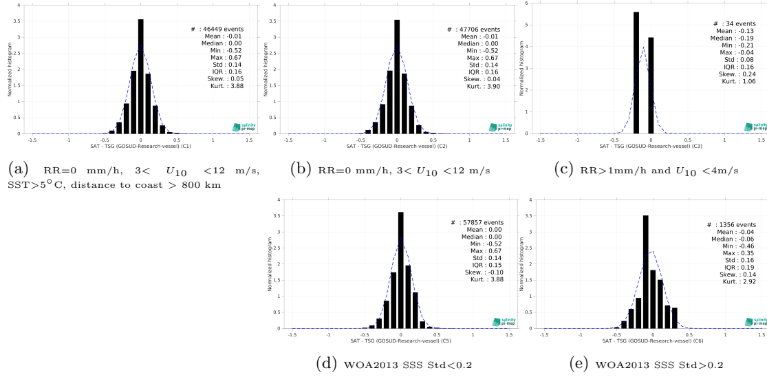
Figure 15: Normalized histogram of \Delta\text{SSS} (SMOS SSS L4 v1 - Daily (CMEMS-CNR) - TSG (GOSUD-Research-vessel)) for 5 different subdatasets corresponding to: RR=0 mm/h, 3 < U_{10} < 12 m/s, SST > 5^\circ\text{C} , distance to coast > 800 km (a), RR=0 mm/h, 3 < U_{10} < 12 m/s (b), RR > 1 mm/h and U_{10} < 4 m/s (c), WOA2013 SSS Std < 0.2 (d), WOA2013 SSS Std > 0.2 (e).
