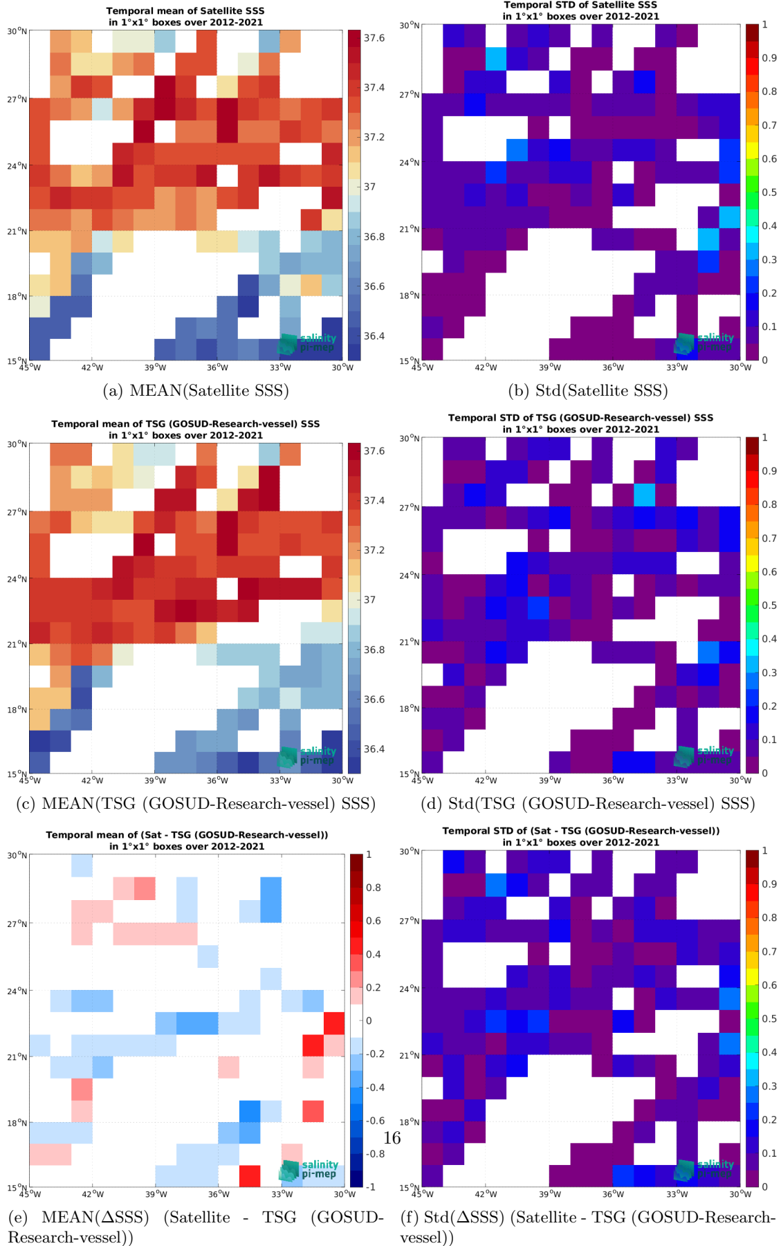
Figure 7: Temporal mean (left) and Std (right) of SSS from SMOS SSS L4 v1 - Daily (CMEMS-CNR) (top), TSG (GOSUD-Research-vessel) (middle), and of \Delta SSS (Satellite - TSG (GOSUD-Research-vessel)). Only match-up pairs are used to generate these maps.
