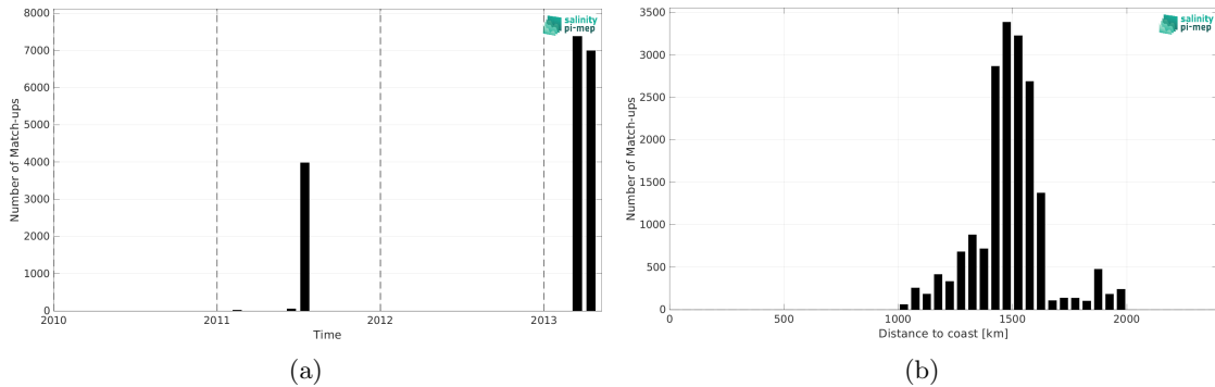
Figure 2: Number of match-ups between TSG (CSIC-UTM) and SMOS SSS L4 v1 - Daily (CMEMS-CNR) SSS as a function of time (a) and as function of the distance to coast (b) over the SPURS 1 Pi-MEP region and for the full satellite product period.
