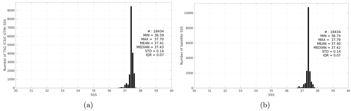
Figure 3: Histograms of SSS from TSG (CSIC-UTM) (a) and SMOS SSS L4 v1 - Daily (CMEMS-CNR) (b) considering all match-up pairs per bins of 0.1 over the SPURS 1 Pi-MEP region and for the full satellite product period.
