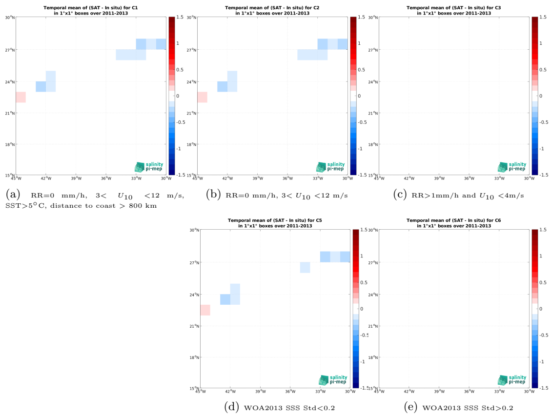
Figure 14: Temporal mean gridded over spatial boxes of size 1^\circ \times 1^\circ of \Delta SSS (SMOS SSS L4 v1 - Daily (CMEMS-CNR) - TSG (CSIC-UTM)) for 5 different subdatasets corresponding to: RR=0 mm/h, 3 < U_{10} < 12 m/s, SST > 5^\circ C , distance to coast > 800 km (a), RR=0 mm/h, 3 < U_{10} < 12 m/s (b), RR > 1 mm/h and U_{10} < 4 m/s (c), WOA2013 SSS Std < 0.2 (d), WOA2013 SSS Std > 0.2 (e).
