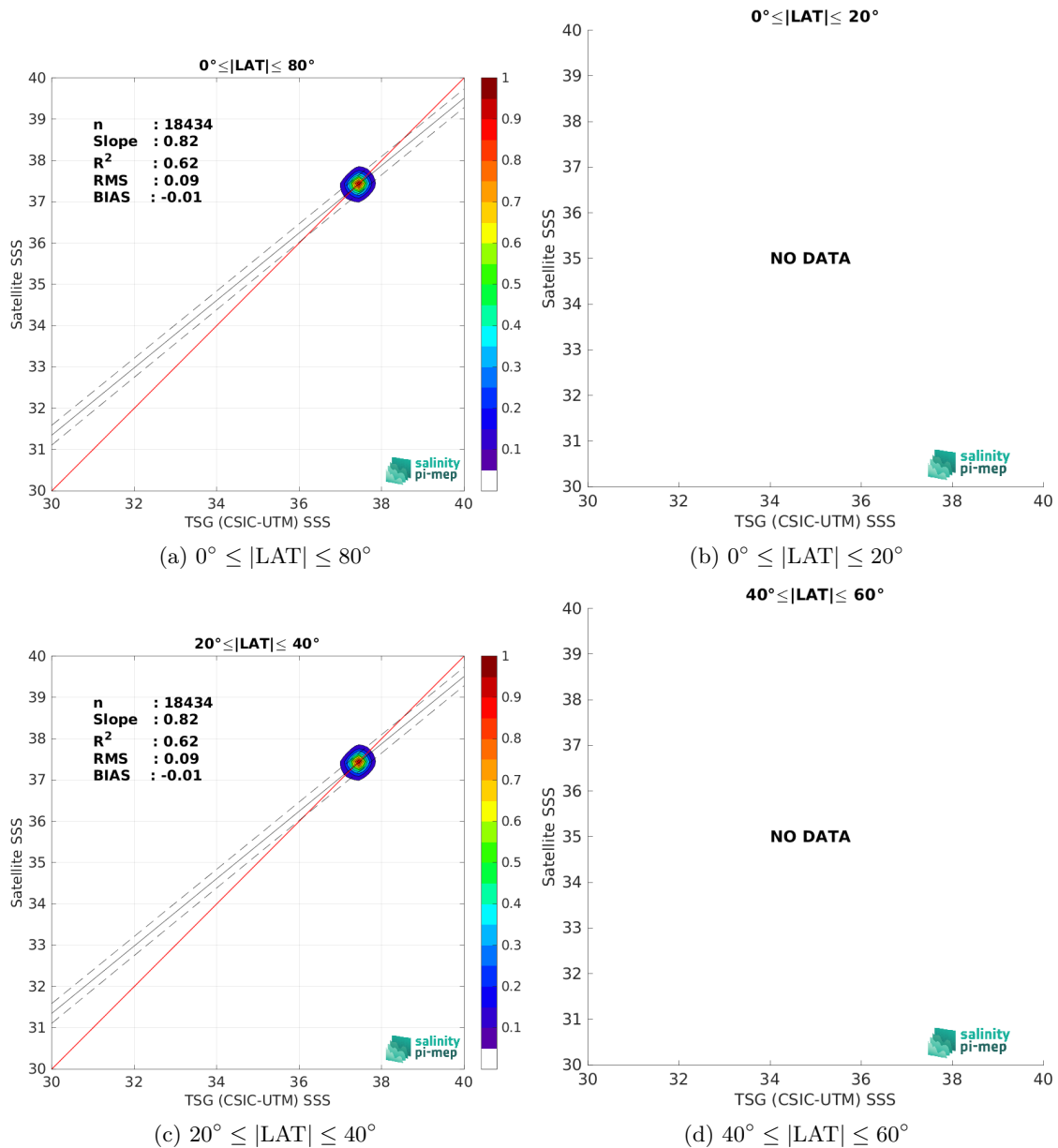
Figure 10: Contour maps of the concentration of SMOS SSS L4 v1 - Daily (CMEMS-CNR) SSS (y-axis) versus TSG (CSIC-UTM) SSS (x-axis) at match-up pairs for different latitude bands. For each plot, the red line shows x=y . The black thin and dashed lines indicate a linear fit through the data cloud and the \pm 95\% confidence levels, respectively. The number match-up pairs n , the slope and R^2 coefficient of the linear fit, the root mean square (RMS) and the mean bias between satellite and in situ data are indicated for each latitude band in each plots.
