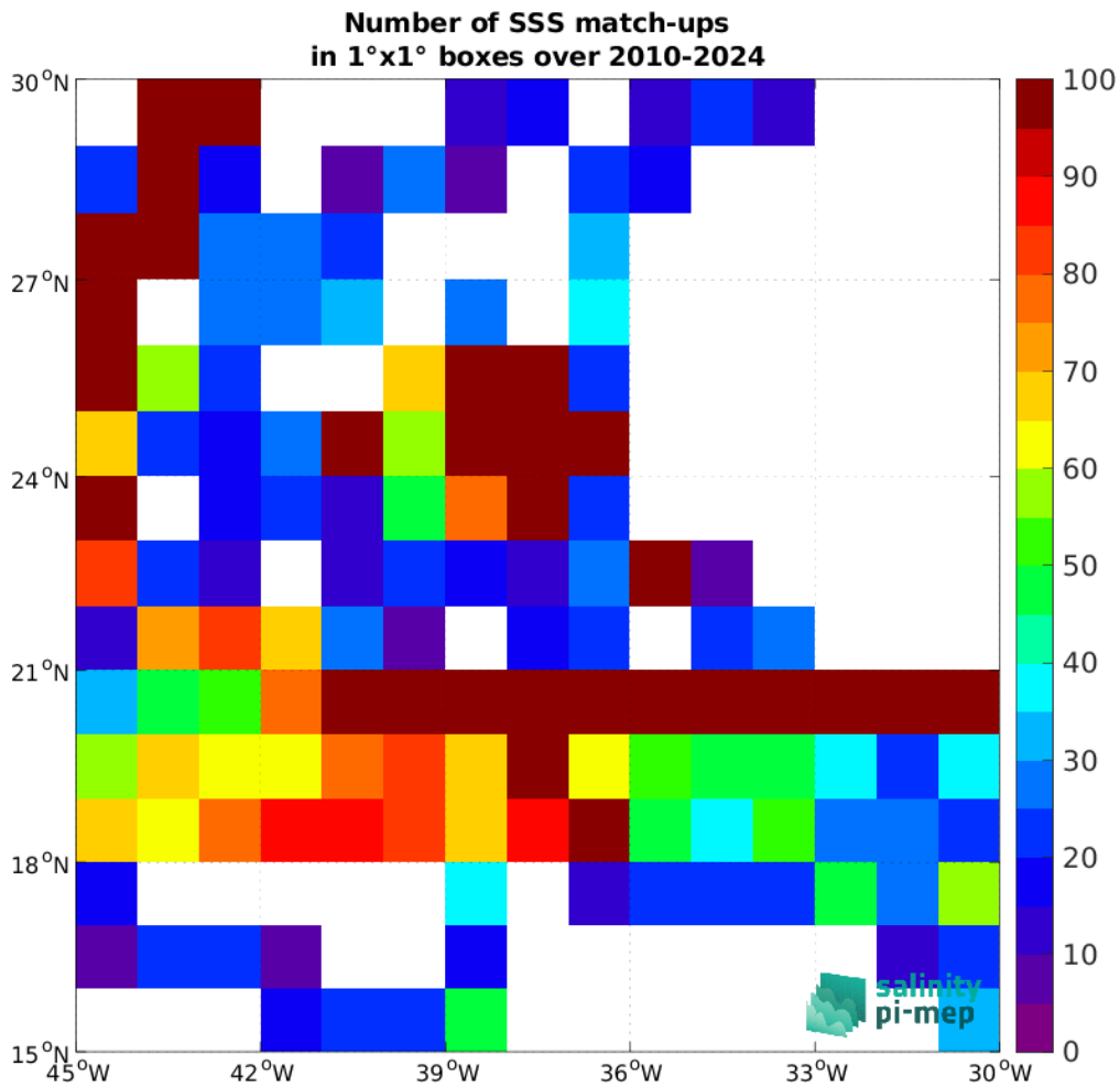
Figure 5: Number of SSS match-ups between TSG (SAMOS) SSS and the SMOS SSS L4 OI v346 - Weekly (CMEMS-CATDS-LOPS) SSS product for the SPURS 1 Pi-MEP region over 1°x1° boxes and for the full satellite product period.
