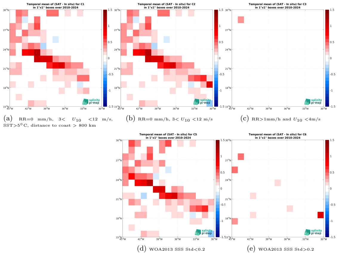
Figure 14: Temporal mean gridded over spatial boxes of size 1^\circ \times 1^\circ of \Delta SSS (SMOS SSS L4 OI v346 - Weekly (CMEMS-CATDS-LOPS) - TSG (SAMOS)) for 5 different subdatasets corresponding to:RR=0 mm/h, 3 < U_{10} < 12 m/s, SST >5^\circ C, distance to coast > 800 km (a), RR=0 mm/h, 3 < U_{10} < 12 m/s (b), RR >1 mm/h and U_{10} < 4 m/s (c), WOA2013 SSS Std <0.2 (d), WOA2013 SSS Std >0.2 (e).
