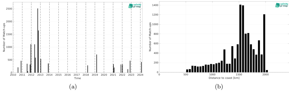
Figure 2: Number of match-ups between TSG (SAMOS) and SMOS SSS L4 OI v346 - Weekly (CMEMS-CATDS-LOPS) SSS as a function of time (a) and as function of the distance to coast (b) over the SPURS 1 Pi-MEP region and for the full satellite product period.
