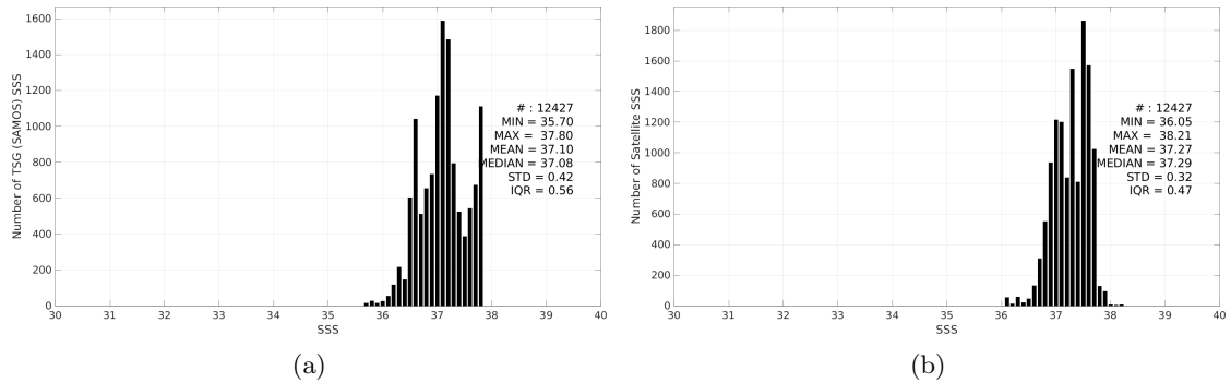
Figure 3: Histograms of SSS from TSG (SAMOS) (a) and SMOS SSS L4 OI v346 - Weekly (CMEMS-CATDS-LOPS) (b) considering all match-up pairs per bins of 0.1 over the SPURS 1 Pi-MEP region and for the full satellite product period.
