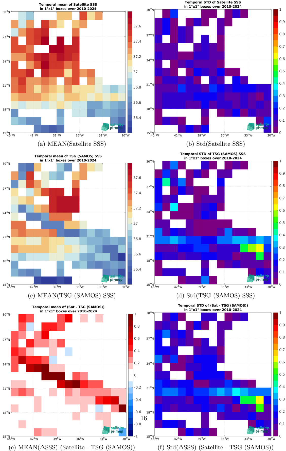
Figure 7: Temporal mean (left) and Std (right) of SSS from SMOS SSS L4 OI v346 - Weekly (CMEMS-CATDS-LOPS) (top), TSG (SAMOS) (middle), and of \Delta SSS (Satellite - TSG (SAMOS)). Only match-up pairs are used to generate these maps.
