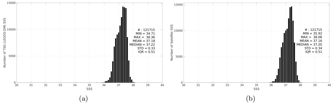
Figure 3: Histograms of SSS from TSG (LEGOS-DM) (a) and SMOS SSS L4 OI v346 - Weekly (CMEMS-CATDS-LOPS) (b) considering all match-up pairs per bins of 0.1 over the SPURS 1 Pi-MEP region and for the full satellite product period.
