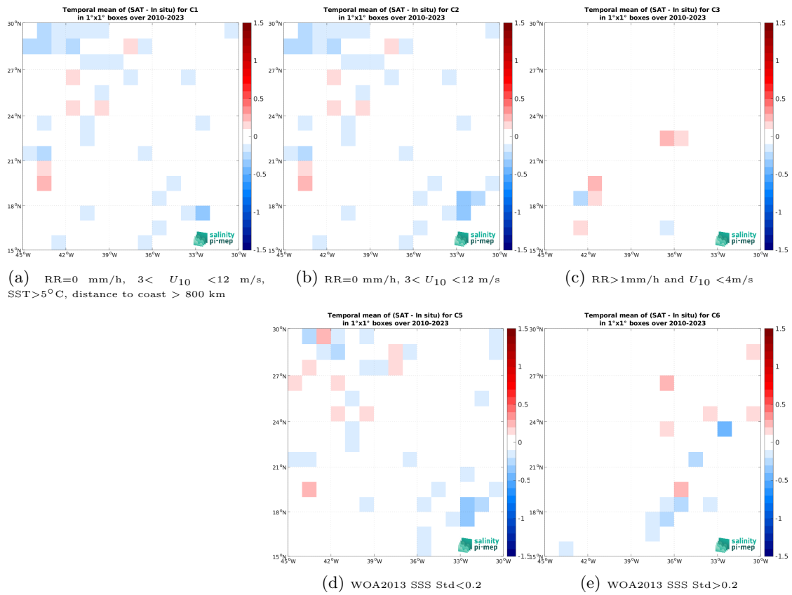
Figure 14: Temporal mean gridded over spatial boxes of size 1^\circ \times 1^\circ of \Delta SSS (SMOS SSS L4 OI v346 - Weekly (CMEMS-CATDS-LOPS) - TSG (LEGOS-DM)) for 5 different subdatasets corresponding to: RR=0 mm/h, 3 < U_{10} < 12 m/s, SST > 5^\circ\text{C} , distance to coast > 800 km (a), RR=0 mm/h, 3 < U_{10} < 12 m/s (b), RR > 1 mm/h and U_{10} < 4 m/s (c), WOA2013 SSS Std < 0.2 (d), WOA2013 SSS Std > 0.2 (e).
