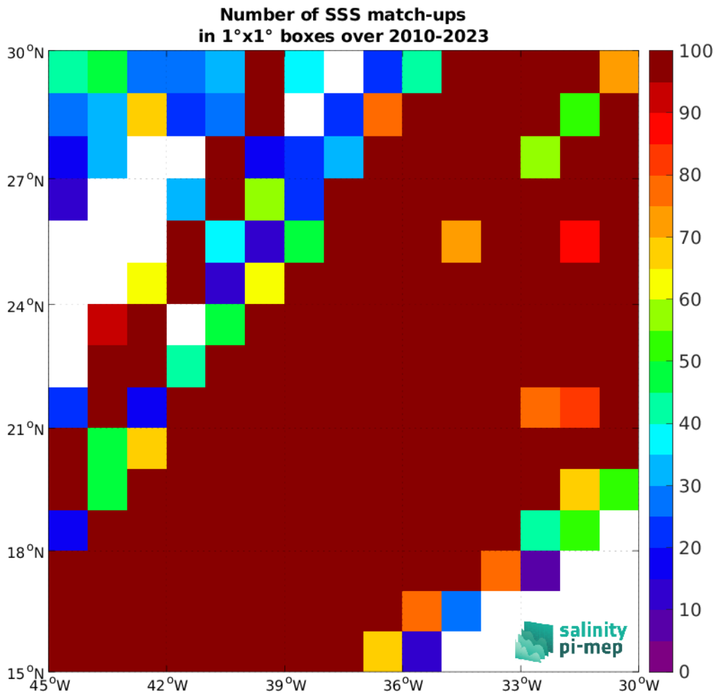
Figure 5: Number of SSS match-ups between TSG (LEGOS-DM) SSS and the SMOS SSS L4 OI v346 - Weekly (CMEMS-CATDS-LOPS) SSS product for the SPURS 1 Pi-MEP region over 1^\circ \times 1^\circ boxes and for the full satellite product period.
