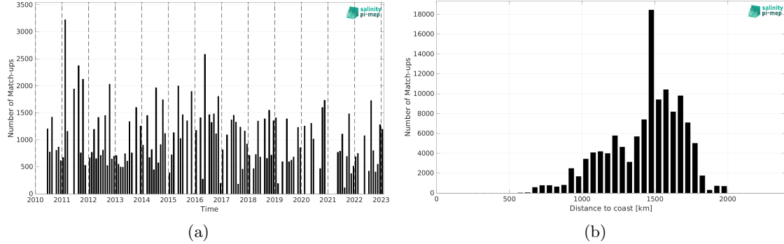
Figure 2: Number of match-ups between TSG (LEGOS-DM) and SMOS SSS L4 OI v346 - Weekly (CMEMS-CATDS-LOPS) SSS as a function of time (a) and as function of the distance to coast (b) over the SPURS 1 Pi-MEP region and for the full satellite product period.
