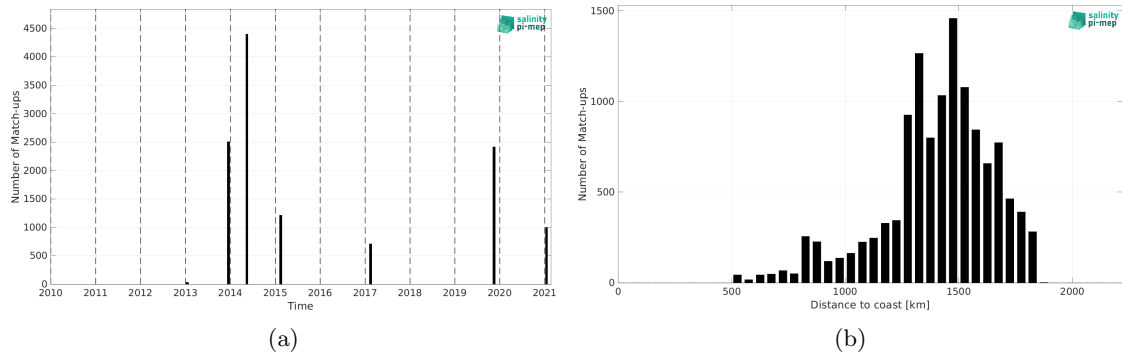
Figure 2: Number of match-ups between TSG (GOSUD-Sailing-ship) and SMOS SSS L4 OI v346 - Weekly (CMEMS-CATDS-LOPS) SSS as a function of time (a) and as function of the distance to coast (b) over the SPURS 1 Pi-MEP region and for the full satellite product period.
