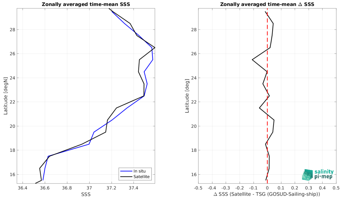
Figure 9: Left panel: Zonal mean SSS from SMOS SSS L4 OI v346 - Weekly (CMEMS-CATDS-LOPS) satellite product (black) and from TSG (GOSUD-Sailing-ship) (blue). Right panel: Zonal mean of \Delta SSS (Satellite - TSG (GOSUD-Sailing-ship)) for all the collected Pi-MEP match-up pairs estimated over the full satellite product period.
