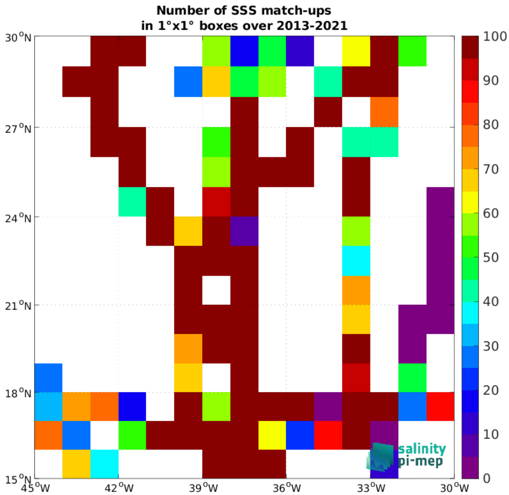
Figure 5: Number of SSS match-ups between TSG (GOSUD-Sailing-ship) SSS and the SMOS SSS L4 OI v346 - Weekly (CMEMS-CATDS-LOPS) SSS product for the SPURS 1 Pi-MEP region over 1°x1° boxes and for the full satellite product period.
