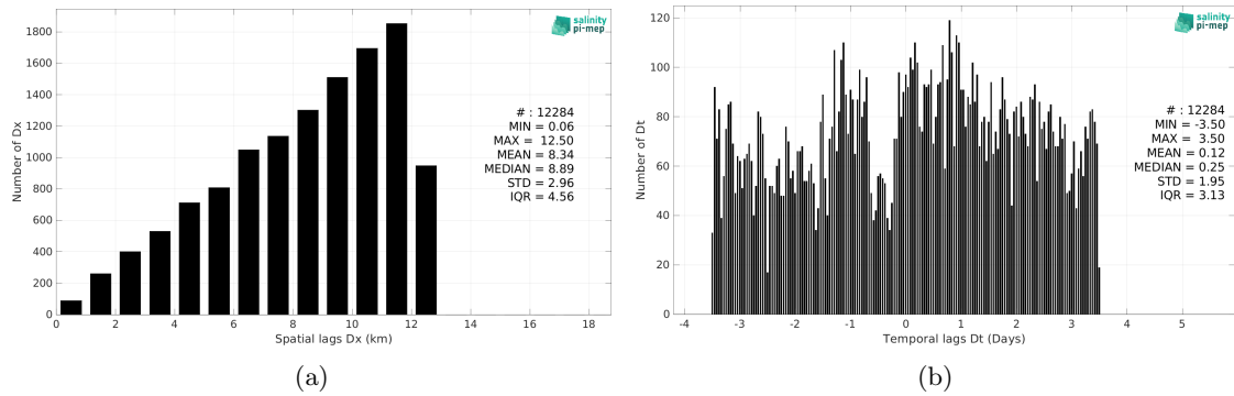
Figure 6: Histograms of the spatial (a) and temporal (b) lags between the location/time of the TSG (GOSUD-Sailing-ship) measurement and the date of the corresponding SMOS SSS L4 OI v346 - Weekly (CMEMS-CATDS-LOPS) SSS pixel.
