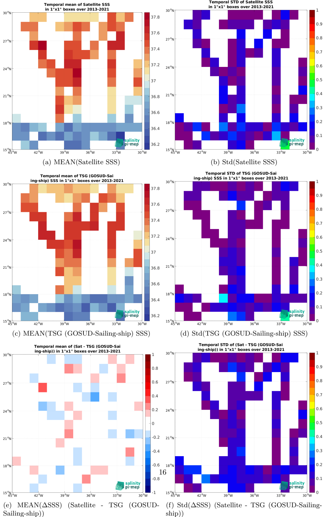
Figure 7: Temporal mean (left) and Std (right) of SSS from SMOS SSS L4 OI v346 - Weekly (CMEMS-CATDS-LOPS) (top), TSG (GOSUD-Sailing-ship) (middle), and of \Delta SSS (Satellite - TSG (GOSUD-Sailing-ship)). Only match-up pairs are used to generate these maps.
