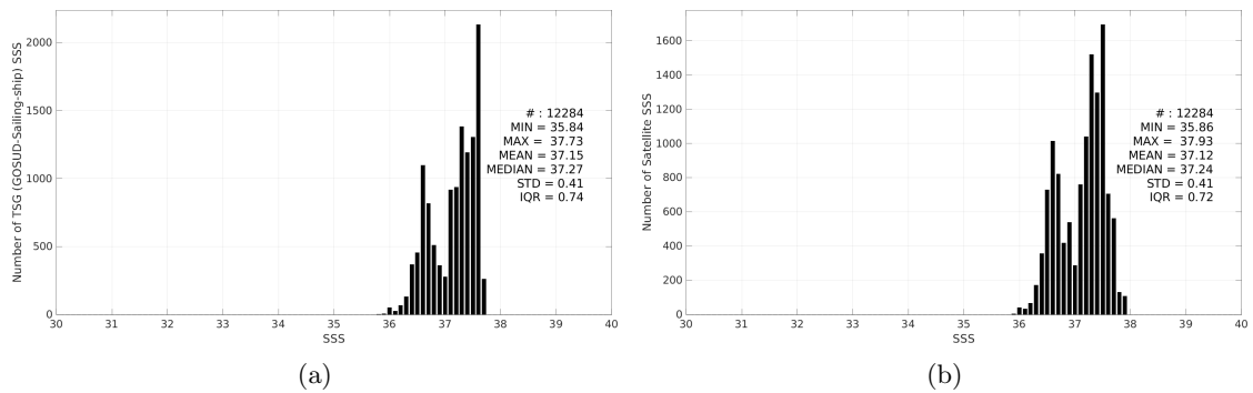
Figure 3: Histograms of SSS from TSG (GOSUD-Sailing-ship) (a) and SMOS SSS L4 OI v346 - Weekly (CMEMS-CATDS-LOPS) (b) considering all match-up pairs per bins of 0.1 over the SPURS 1 Pi-MEP region and for the full satellite product period.
