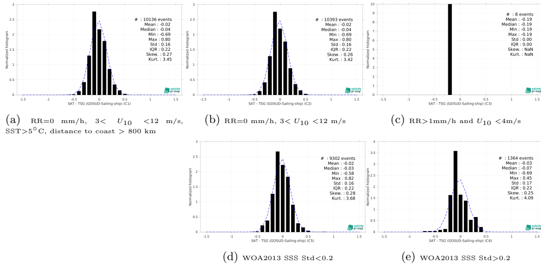
Figure 15: Normalized histogram of \Delta\text{SSS} (SMOS SSS L4 OI v346 - Weekly (CMEMS-CATDS-LOPS) - TSG (GOSUD-Sailing-ship)) for 5 different subdatasets corresponding to: RR=0 mm/h, 3 < U_{10} < 12 m/s, SST > 5^\circ\text{C} , distance to coast > 800 km (a), RR=0 mm/h, 3 < U_{10} < 12 m/s (b), RR > 1\text{mm/h} and U_{10} < 4\text{m/s} (c), WOA2013 SSS Std < 0.2 (d), WOA2013 SSS Std > 0.2 (e).
