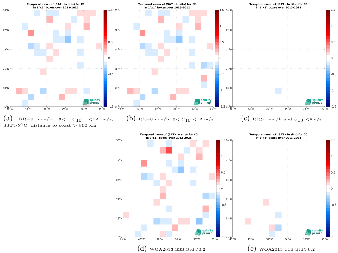
Figure 14: Temporal mean gridded over spatial boxes of size 1^\circ \times 1^\circ of \Delta SSS (SMOS SSS L4 OI v346 - Weekly (CMEMS-CATDS-LOPS) - TSG (GOSUD-Sailing-ship)) for 5 different sub-datasets corresponding to:RR=0 mm/h, 3 < U_{10} < 12 m/s, SST >5^\circ C, distance to coast > 800 km (a), RR=0 mm/h, 3 < U_{10} < 12 m/s (b), RR >1 mm/h and U_{10} < 4 m/s (c), WOA2013 SSS Std <0.2 (d), WOA2013 SSS Std >0.2 (e).
