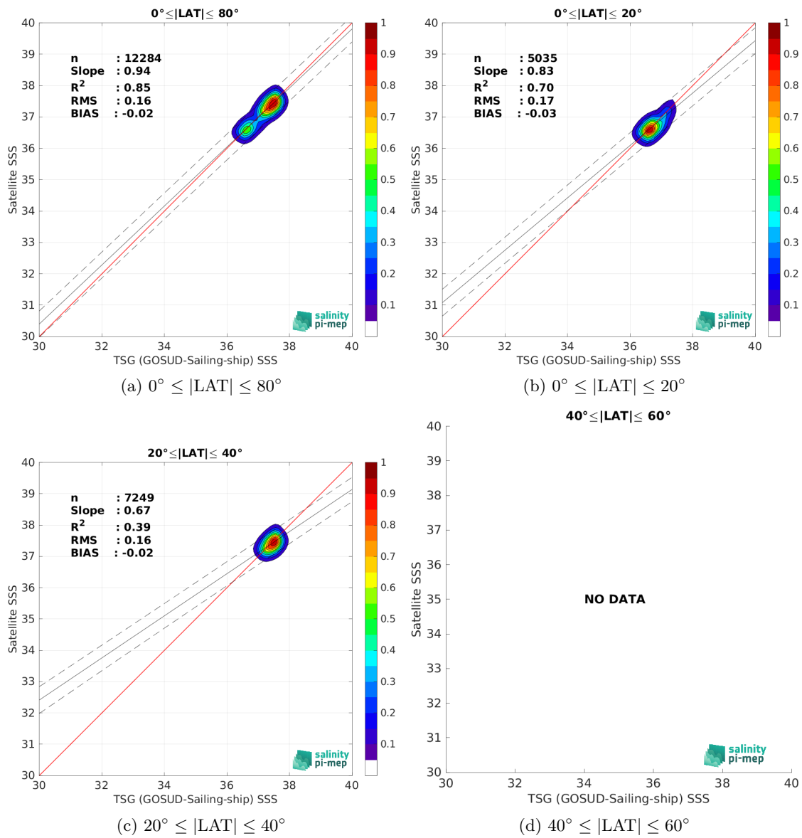
Figure 10: Contour maps of the concentration of SMOS SSS L4 OI v346 - Weekly (CMEMS-CATDS-LOPS) SSS (y-axis) versus TSG (GOSUD-Sailing-ship) SSS (x-axis) at match-up pairs for different latitude bands. For each plot, the red line shows x=y . The black thin and dashed lines indicate a linear fit through the data cloud and the \pm 95\% confidence levels, respectively. The number match-up pairs n , the slope and R^2 coefficient of the linear fit, the root mean square (RMS) and the mean bias between satellite and in situ data are indicated for each latitude band in each plots.
