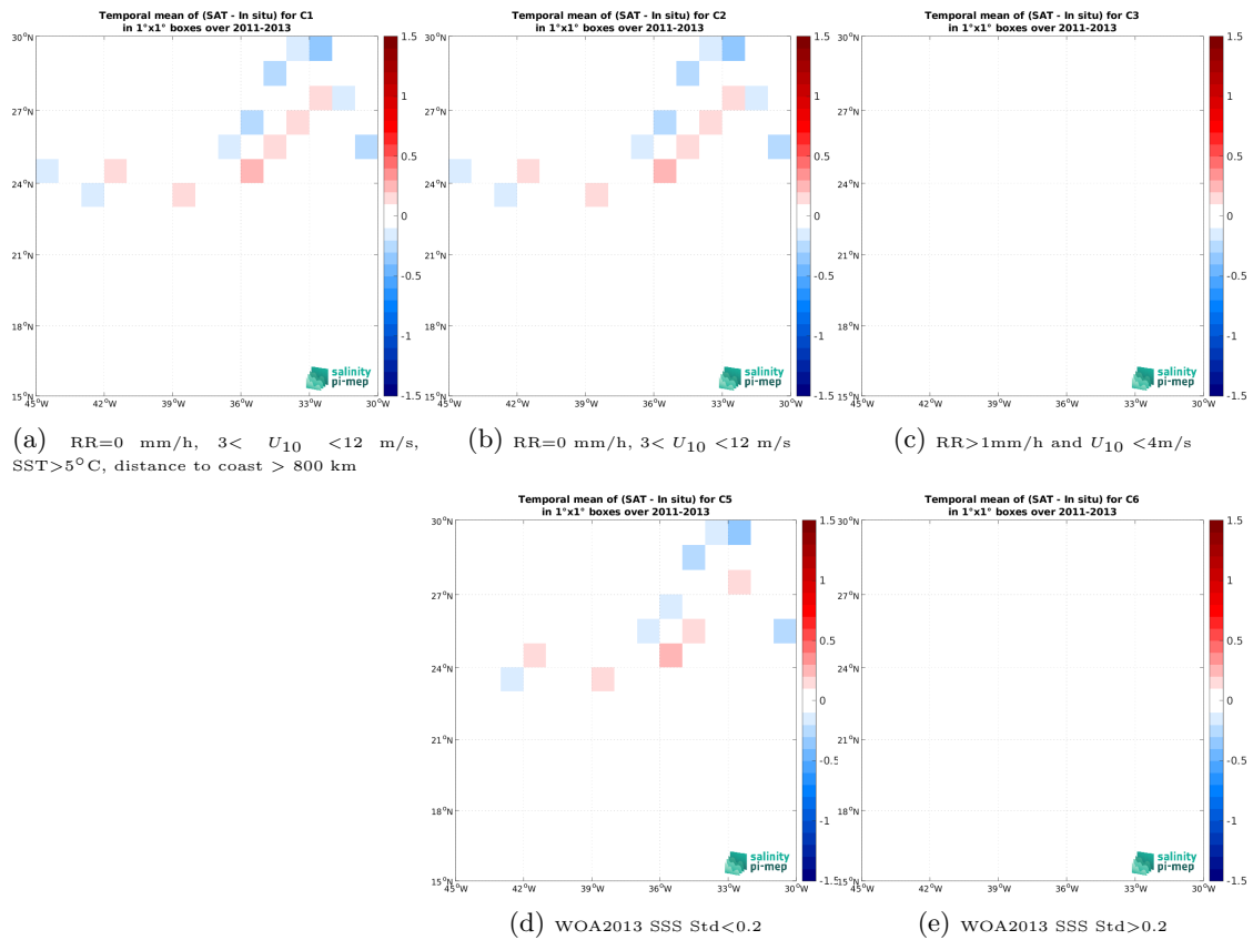
Figure 14: Temporal mean gridded over spatial boxes of size 1^\circ \times 1^\circ of \Delta SSS (SMOS SSS L4 OI v346 - Weekly (CMEMS-CATDS-LOPS) - TSG (CSIC-UTM)) for 5 different subdatasets corresponding to: RR=0 mm/h, 3 < U_{10} < 12 m/s, SST > 5^\circ C , distance to coast > 800 km (a), RR=0 mm/h, 3 < U_{10} < 12 m/s (b), RR > 1 mm/h and U_{10} < 4 m/s (c), WOA2013 SSS Std < 0.2 (d), WOA2013 SSS Std > 0.2 (e).
