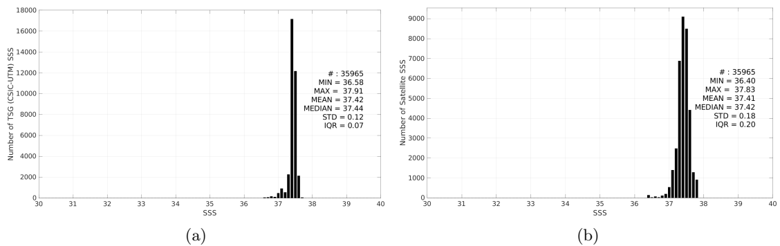
Figure 3: Histograms of SSS from TSG (CSIC-UTM) (a) and SMOS SSS L4 OI v346 - Weekly (CMEMS-CATDS-LOPS) (b) considering all match-up pairs per bins of 0.1 over the SPURS 1 Pi-MEP region and for the full satellite product period.
