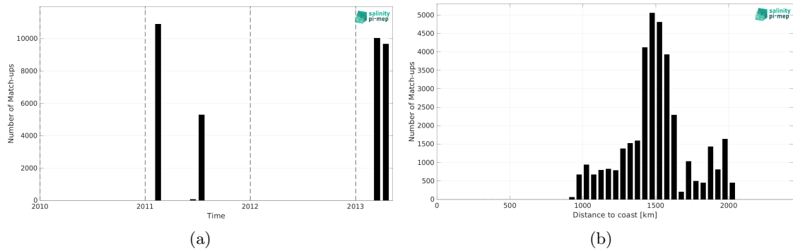
Figure 2: Number of match-ups between TSG (CSIC-UTM) and SMOS SSS L4 OI v346 - Weekly (CMEMS-CATDS-LOPS) SSS as a function of time (a) and as function of the distance to coast (b) over the SPURS 1 Pi-MEP region and for the full satellite product period.
