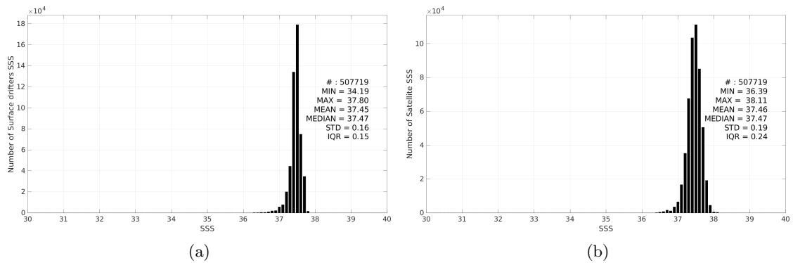
Figure 3: Histograms of SSS from Surface drifters (a) and SMOS SSS L4 OI v346 - Weekly (CMEMS-CATDS-LOPS) (b) considering all match-up pairs per bins of 0.1 over the SPURS 1 Pi-MEP region and for the full satellite product period.
