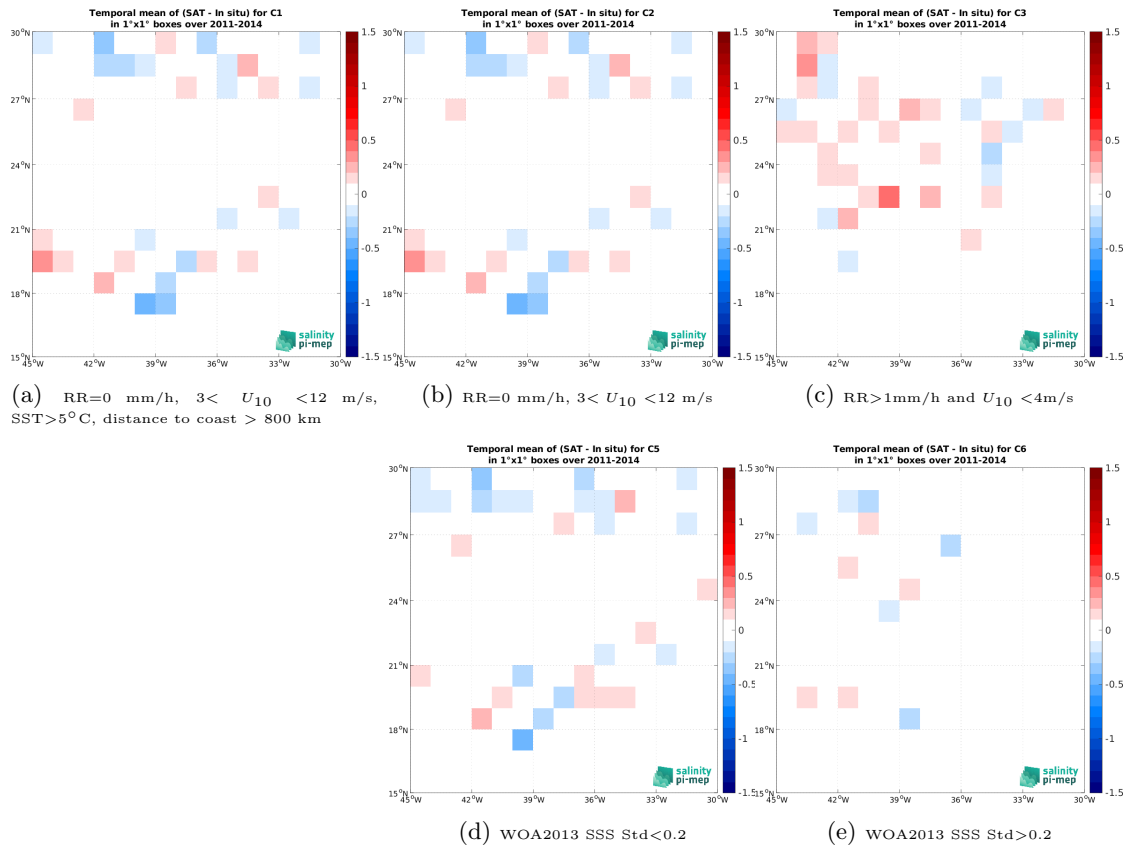
Figure 13: Temporal mean gridded over spatial boxes of size 1^\circ \times 1^\circ of \Delta SSS (SMOS SSS L4 OI v346 - Weekly (CMEMS-CATDS-LOPS) - Surface drifters) for 5 different subdatasets corresponding to:RR=0 mm/h, 3 < U_{10} < 12 m/s, SST >5^\circ C, distance to coast > 800 km (a), RR=0 mm/h, 3 < U_{10} < 12 m/s (b), RR >1 mm/h and U_{10} < 4 m/s (c), WOA2013 SSS Std <0.2 (d), WOA2013 SSS Std >0.2 (e).
