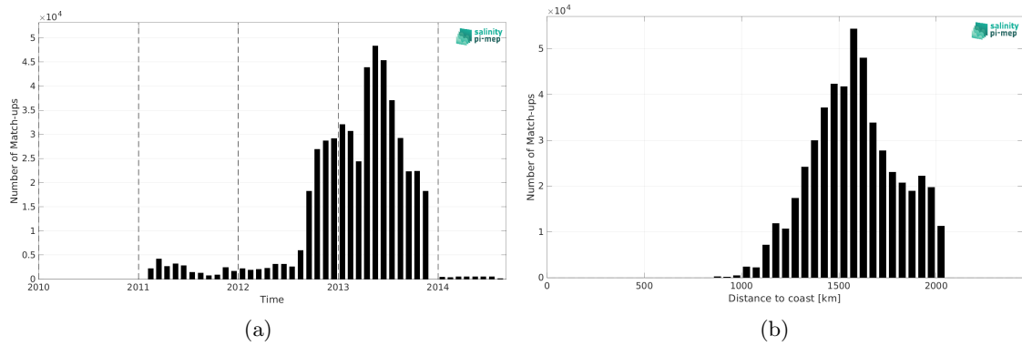
Figure 2: Number of match-ups between Surface drifters and SMOS SSS L4 OI v346 - Weekly (CMEMS-CATDS-LOPS) SSS as a function of time (a) and as function of the distance to coast (b) over the SPURS 1 Pi-MEP region and for the full satellite product period.
