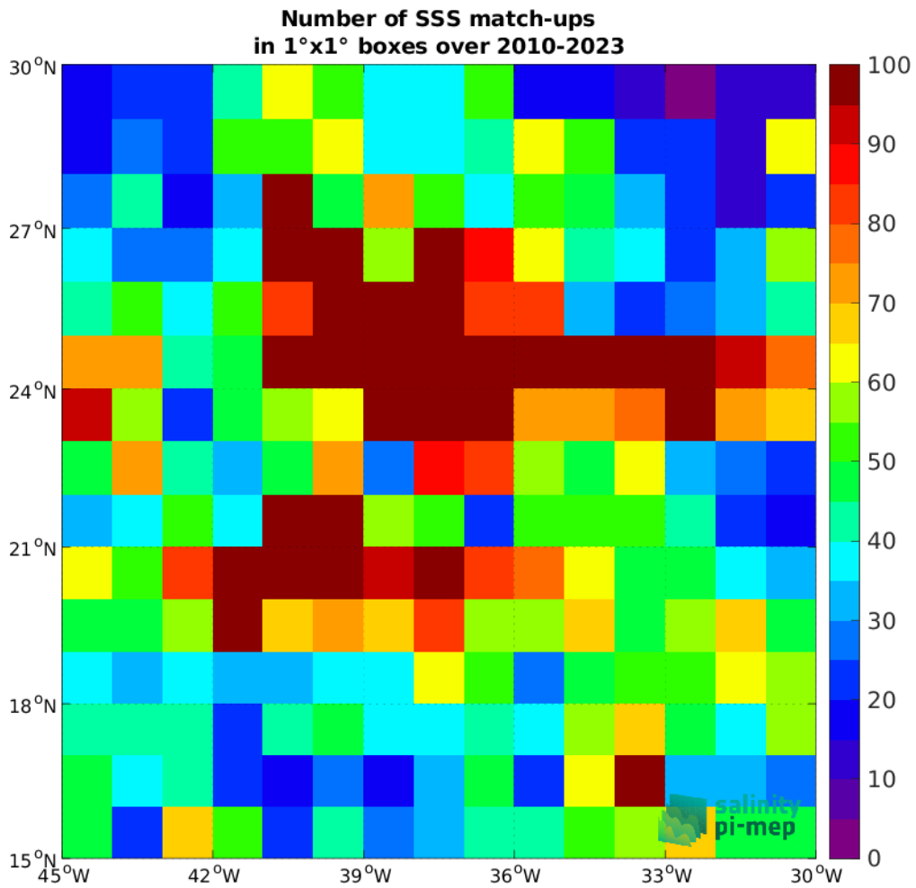
Figure 5: Number of SSS match-ups between Argo SSS and the SMOS SSS L4 OI v346 - Weekly (CMEMS-CATDS-LOPS) SSS product for the SPURS 1 Pi-MEP region over 1°x1° boxes and for the full satellite product period.
