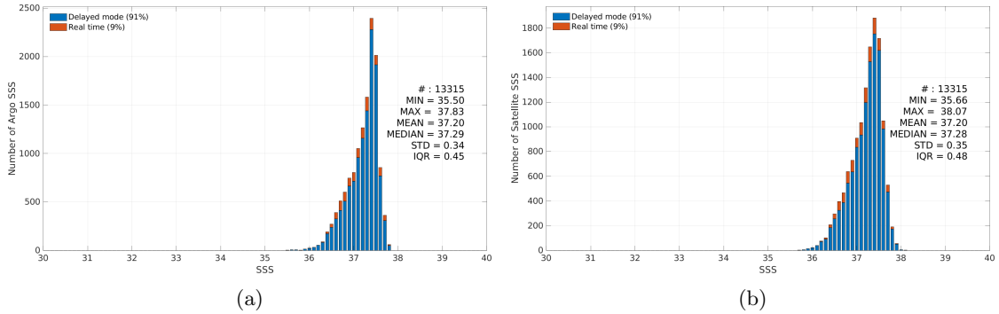
Figure 3: Histograms of SSS from Argo (a) and SMOS SSS L4 OI v346 - Weekly (CMEMS-CATDS-LOPS) (b) considering all match-up pairs per bins of 0.1 over the SPURS 1 Pi-MEP region and for the full satellite product period.
