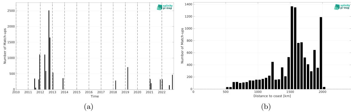
Figure 1: Number of match-ups between TSG (SAMOS) and SMOS SSS L4 OI v342 - Weekly (CMEMS-CATDS-LOPS) SSS as a function of time (a) and as function of the distance to coast (b) over the SPURS 1 Pi-MEP region and for the full satellite product period.
