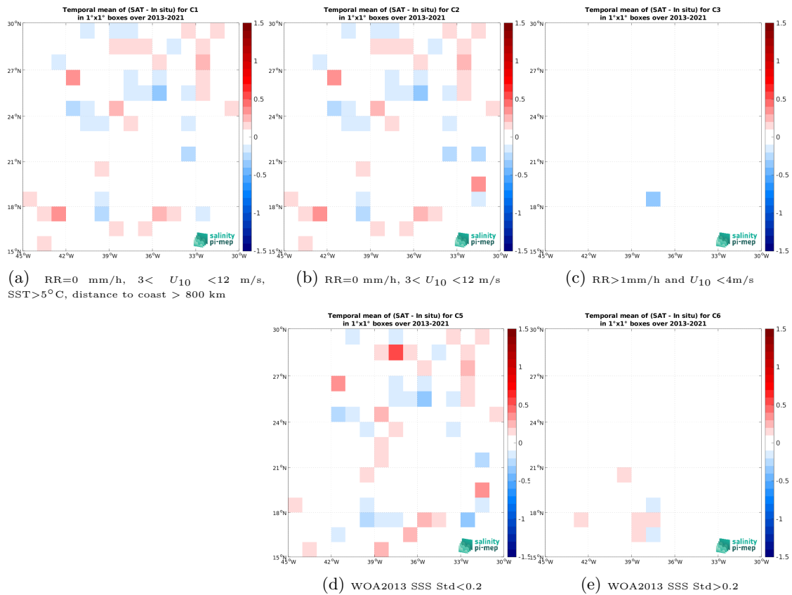
Figure 12: Temporal mean gridded over spatial boxes of size 1^{\circ} \times 1^{\circ} of \Delta\text{SSS} (SMOS SSS L4 OI v342 - Weekly (CMEMS-CATDS-LOPS) - TSG (GOSUD-Sailing-ship)) for 5 different sub-datasets corresponding to: RR=0 mm/h, 3 < U_{10} < 12 m/s, SST > 5^{\circ}\text{C} , distance to coast > 800 km (a), RR=0 mm/h, 3 < U_{10} < 12 m/s (b), RR > 1\text{mm/h} and U_{10} < 4\text{m/s} (c), WOA2013 SSS Std < 0.2 (d), WOA2013 SSS Std > 0.2 (e).
