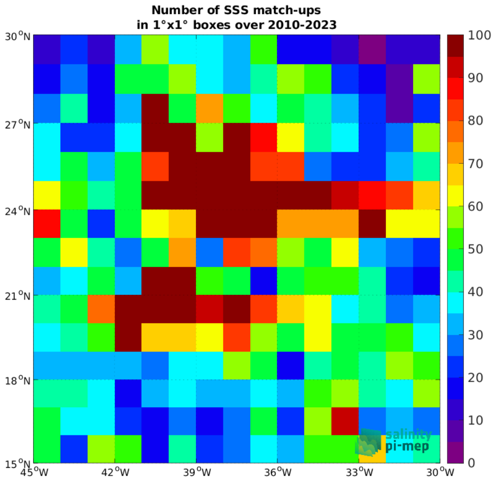
Figure 4: Number of SSS match-ups between Argo SSS and the SMOS SSS L4 OI v342 - Weekly (CMEMS-CATDS-LOPS) SSS product for the SPURS 1 Pi-MEP region over 1^\circ \times 1^\circ boxes and for the full satellite product period.
