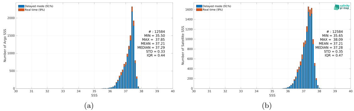
Figure 2: Histograms of SSS from Argo (a) and SMOS SSS L4 OI v342 - Weekly (CMEMS-CATDS-LOPS) (b) considering all match-up pairs per bins of 0.1 over the SPURS 1 Pi-MEP region and for the full satellite product period.
