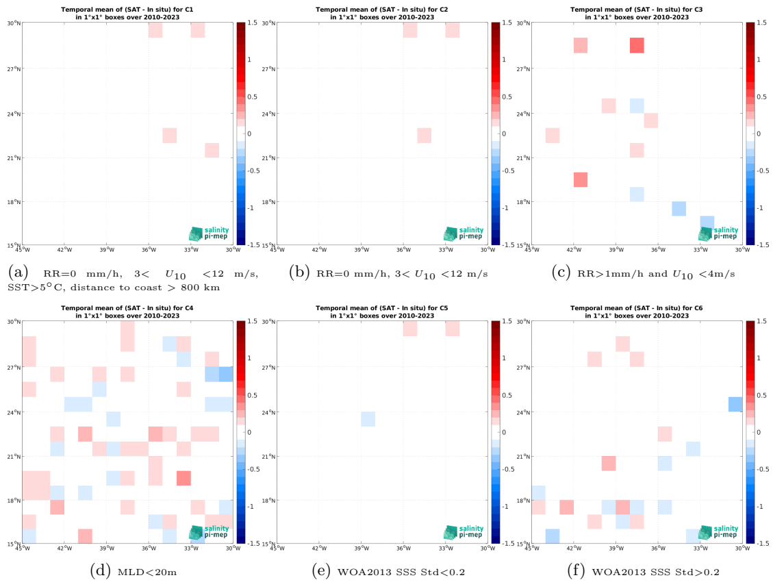
Figure 12: Temporal mean gridded over spatial boxes of size 1^\circ \times 1^\circ of \Delta SSS (SMOS SSS L4 OI v342 - Weekly (CMEMS-CATDS-LOPS) - Argo) for 6 different subdatasets corresponding to:RR=0 mm/h, 3 < U_{10} < 12 m/s, SST >5^\circ C, distance to coast > 800 km (a), RR=0 mm/h, 3 < U_{10} < 12 m/s (b), RR >1 mm/h and U_{10} < 4 m/s (c),MLD <20 m (d),WOA2013 SSS Std <0.2 (e),WOA2013 SSS Std >0.2 (f).
