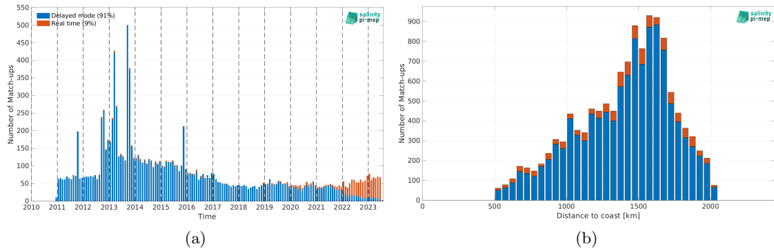
Figure 1: Number of match-ups between Argo and SMOS SSS L4 OI v342 - Weekly (CMEMS-CATDS-LOPS) SSS as a function of time (a) and as function of the distance to coast (b) over the SPURS 1 Pi-MEP region and for the full satellite product period.
