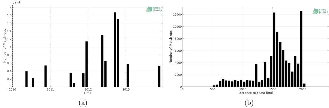
Figure 1: Number of match-ups between TSG (SAMOS) and SMOS L4 v2 Weekly (CATDS-CECOS-IFREMER) SSS as a function of time (a) and as function of the distance to coast (b) over the SPURS 1 Pi-MEP region and for the full satellite product period.
