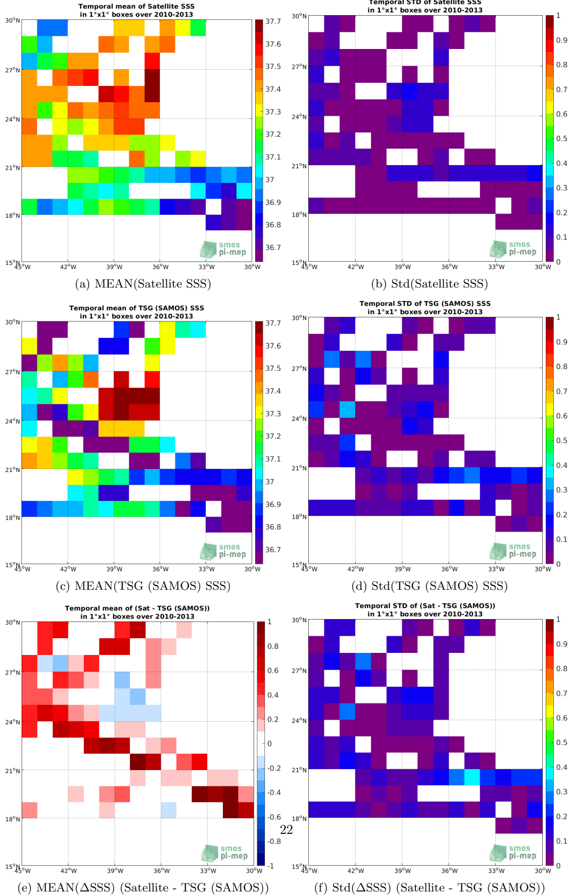
Figure 6: Temporal mean (left) and Std (right) of SSS from SMOS L4 v2 Weekly (CATDS-CECOS-IFREMER) (top), TSG (SAMOS) (middle), and of \Delta SSS (Satellite - TSG (SAMOS)). Only match-up pairs are used to generate these maps.
