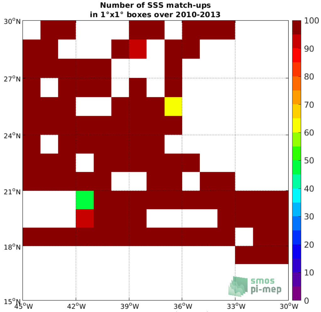
Figure 4: Number of SSS match-ups between TSG (SAMOS) SSS and the SMOS L4 v2 Weekly (CATDS-CECOS-IFREMER) SSS product for the SPURS 1 Pi-MEP region over 1^\circ \times 1^\circ boxes and for the full satellite product period.
