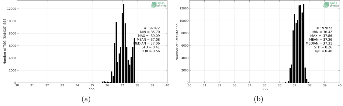
Figure 2: Histograms of SSS from TSG (SAMOS) (a) and SMOS L4 v2 Weekly (CATDS-CECOS-IFREMER) (b) considering all match-up pairs per bins of 0.1 over the SPURS 1 Pi-MEP region and for the full satellite product period.
