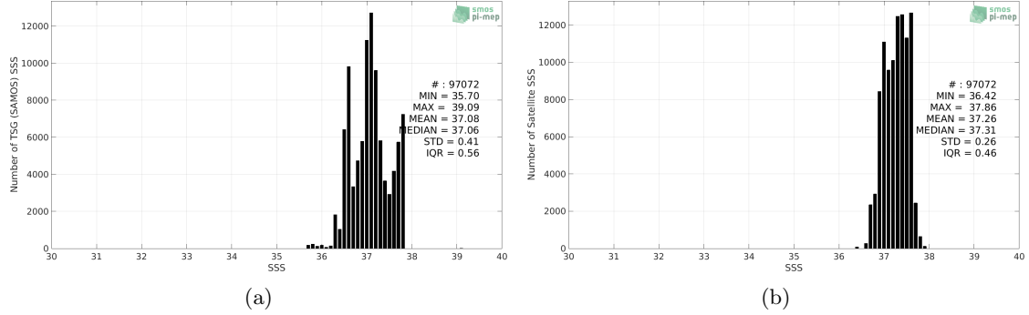
Figure 2: Histograms of SSS from TSG (SAMOS) (a) and SMOS L4 v2 Weekly (CATDS-CECOS-IFREMER) (b) considering all match-up pairs per bins of 0.1 over the SPURS 1 Pi-MEP region and for the full satellite product period.
