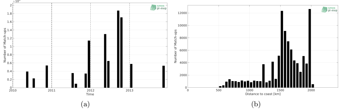
Figure 1: Number of match-ups between TSG (SAMOS) and SMOS L4 v2 Weekly (CATDS-CECOS-IFREMER) SSS as a function of time (a) and as function of the distance to coast (b) over the SPURS 1 Pi-MEP region and for the full satellite product period.
