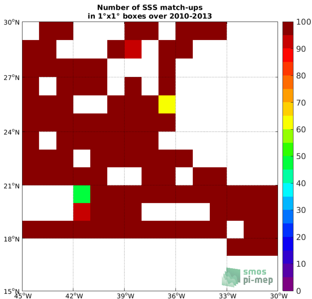
Figure 4: Number of SSS match-ups between TSG (SAMOS) SSS and the SMOS L4 v2 Weekly (CATDS-CECOS-IFREMER) SSS product for the SPURS 1 Pi-MEP region over 1°x1° boxes and for the full satellite product period.
