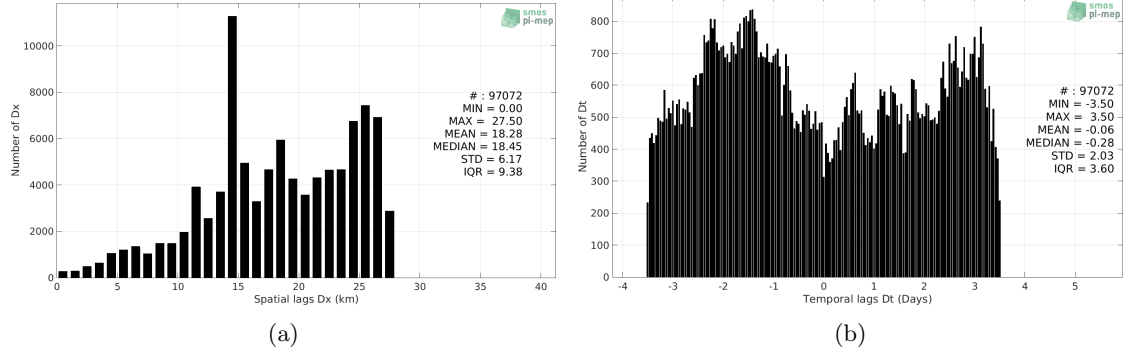
Figure 5: Histograms of the spatial (a) and temporal (b) lags between the time of the TSG (SAMOS) measurements and the date of the corresponding SMOS L4 v2 Weekly (CATDS-CECOS-IFREMER) SSS product.
