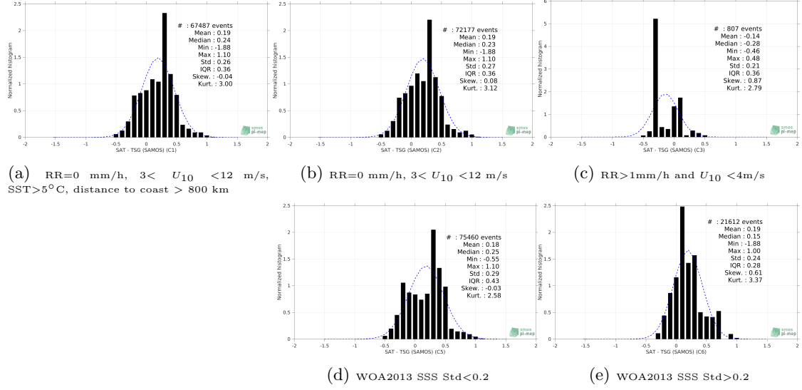
Figure 13: Normalized histogram of \Delta\text{SSS} (SMOS L4 v2 Weekly (CATDS-CECOS-IFREMER) - TSG (SAMOS)) for 5 different subdatasets corresponding to: RR=0 mm/h, 3 < U_{10} < 12 m/s, SST >5^{\circ}\text{C} , distance to coast > 800 km (a), RR=0 mm/h, 3 < U_{10} < 12 m/s (b), RR>1\text{mm/h} and U_{10} < 4\text{m/s} (c), WOA2013 SSS Std <0.2 (d), WOA2013 SSS Std >0.2 (e).
