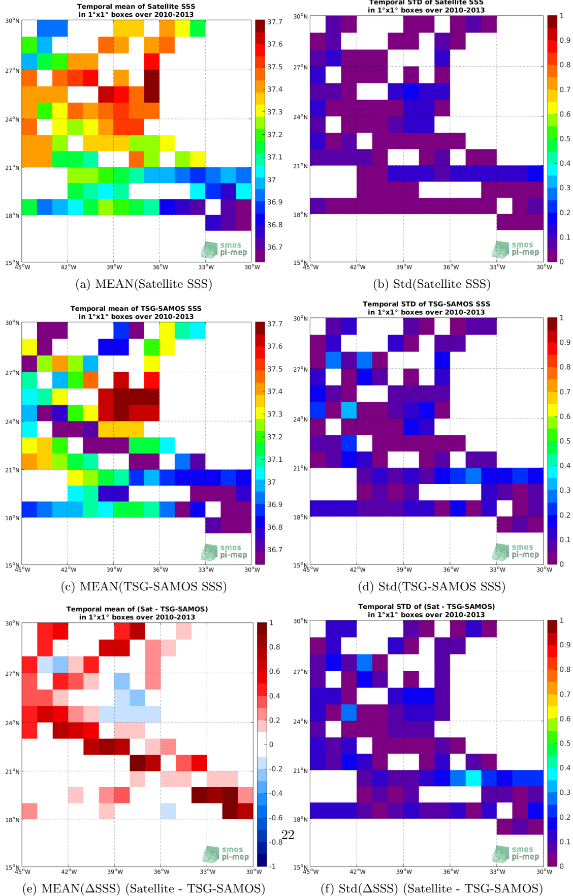
Figure 6: Temporal mean (left) and Std (right) of SSS from SMOS-L4-CATDS-CECOS-IFREMER-V2-WEEKLY-0.5DEG (top), TSG-SAMOS (middle), and of \Delta SSS (Satellite - TSG-SAMOS). Only match-up pairs are used to generate these maps.
