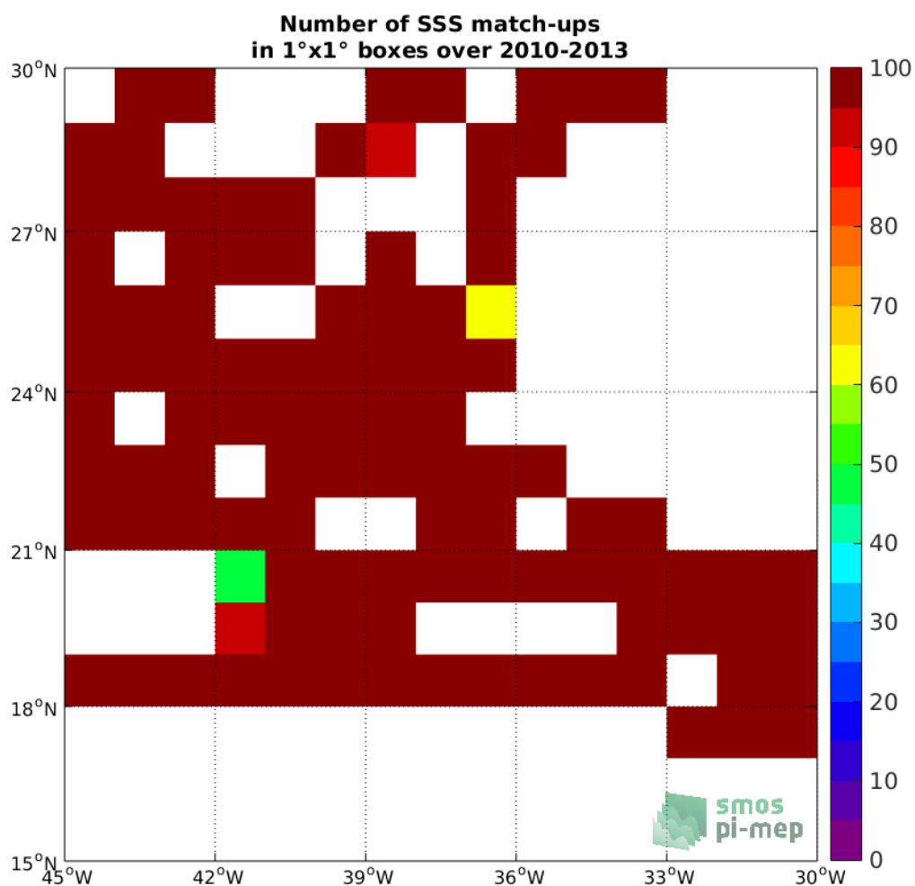
Figure 4: Number of SSS match-ups between TSG-SAMOS SSS and the SMOS-L4-CATDS-CECOS-IFREMER-V2-WEEKLY-0.5DEG SSS product for the SPURS 1 Pi-MEP region over 1°x1° boxes and for the full satellite product period.
