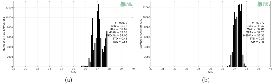
Figure 2: Histograms of SSS from TSG-SAMOS (a) and SMOS-L4-CATDS-CECOS-IFREMER-V2-WEEKLY-0.5DEG (b) considering all match-up pairs per bins of 0.1 over the SPURS 1 Pi-MEP region and for the full satellite product period.
