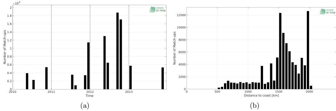
Figure 1: Number of match-ups between TSG-SAMOS and SMOS-L4-CATDS-CECOS-IFREMER-V2-WEEKLY-0.5DEG SSS as a function of time (a) and as function of the distance to coast (b) over the SPURS 1 Pi-MEP region and for the full satellite product period.
