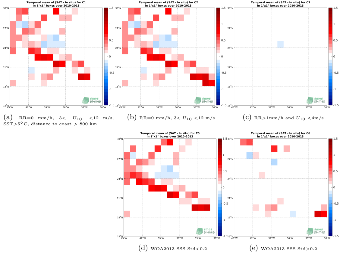
Figure 12: Temporal mean gridded over spatial boxes of size 1^{\circ}\times 1^{\circ} of \Delta\text{SSS} (SMOS-L4-CATDS-CECOS-IFREMER-V2-WEEKLY-0.5DEG - TSG-SAMOS) for 5 different subdatasets corresponding to: RR=0 mm/h, 3 < U_{10} < 12 m/s, SST >5^{\circ}\text{C} , distance to coast > 800 km (a), RR=0 mm/h, 3 < U_{10} < 12 m/s (b), RR >1 mm/h and U_{10} < 4 m/s (c), WOA2013 SSS Std <0.2 (d), WOA2013 SSS Std >0.2 (e).
