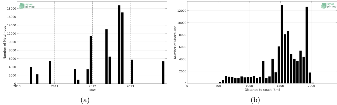
Figure 1: Number of match-ups between TSG-SAMOS and SMOS-L4-CATDS-CECOS-IFREMER-V2-WEEKLY-0.5DEG SSS as a function of time (a) and as function of the distance to coast (b) over the SPURS 1 Pi-MEP region and for the full satellite product period.
