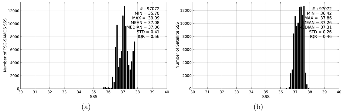
Figure 2: Histograms of SSS from TSG-SAMOS (a) and SMOS-L4-CATDS-CECOS-IFREMER-V2-WEEKLY-0.5DEG (b) considering all match-up pairs per bins of 0.1 over the SPURS 1 Pi-MEP region and for the full satellite product period.
