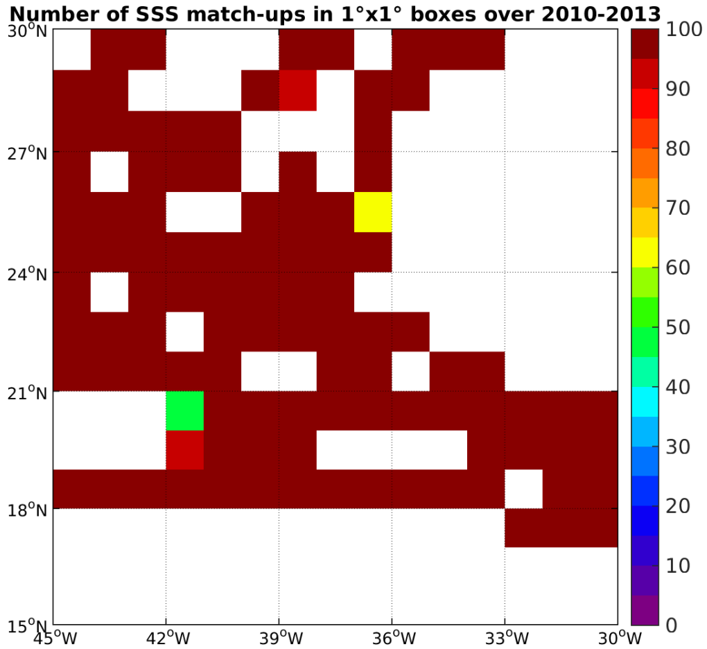
Figure 4: Number of SSS match-ups between TSG-SAMOS SSS and the SMOS-L4-CATDS-CECOS-IFREMER-V2-WEEKLY-0.5DEG SSS product for the SPURS 1 Pi-MEP region over 1°x1° boxes and for the full satellite product period.
