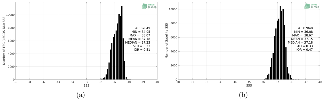
Figure 2: Histograms of SSS from TSG (LEGOS-DM) (a) and SMOS L4 v2 Weekly (CATDS-CECOS-IFREMER) (b) considering all match-up pairs per bins of 0.1 over the SPURS 1 Pi-MEP region and for the full satellite product period.
